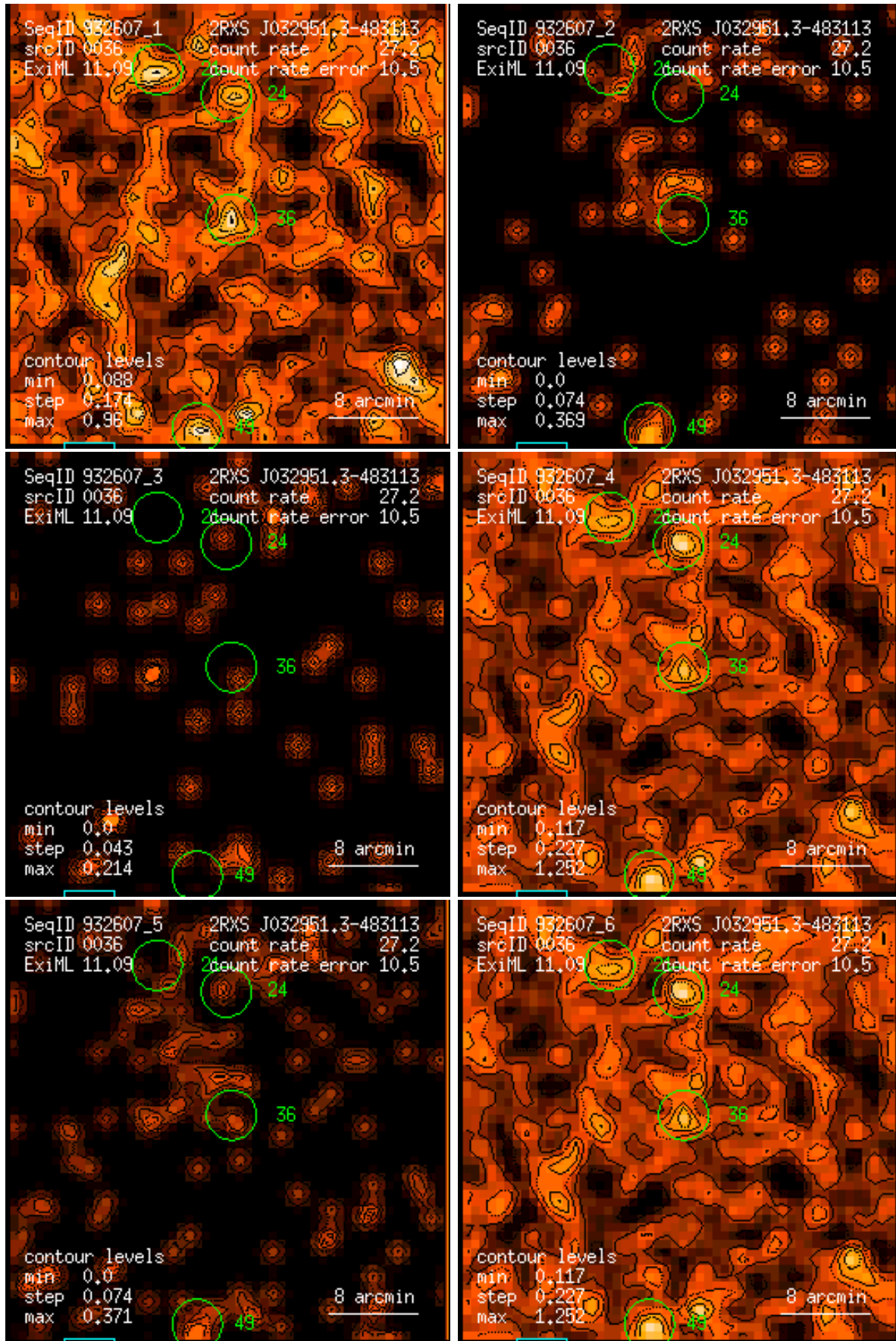
Figure 36: RASS 932607: detection 0036: band rate images, Gaussian filter: (1) PSPC channels 11 – 41, (2) 52 – 90, (3) 91 – 201, (4) 11 – 235, (5) 52 – 201, (6) 11 – 201. Broad band rates in counts/ks. Band rate contour levels in counts/ks/arcmin 2 .
