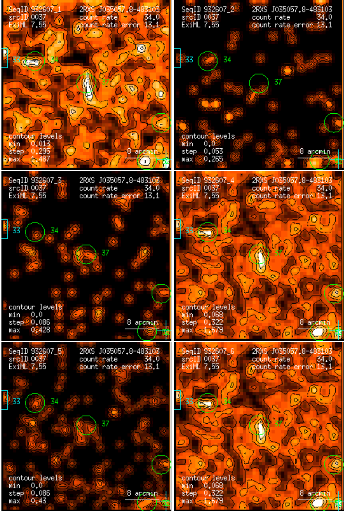
Figure 37: RASS 932607: detection 0037: band rate images, Gaussian filter: (1) PSPC channels 11 – 41, (2) 52 – 90, (3) 91 – 201, (4) 11 – 235, (5) 52 – 201, (6) 11 – 201. Broad band rates in counts/ks. Band rate contour levels in counts/ks/arcmin 2 .
