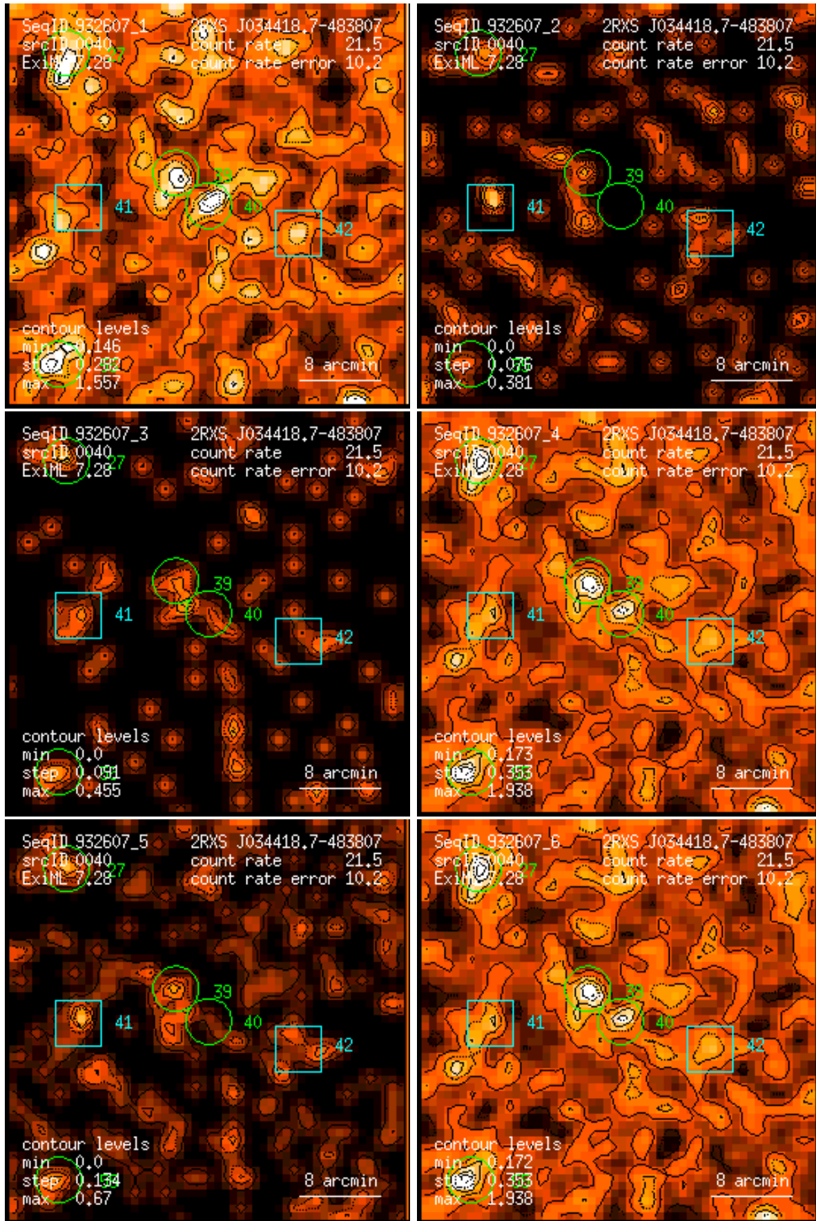
Figure 40: RASS 932607: detection 0040: band rate images, Gaussian filter: (1) PSPC channels 11 – 41, (2) 52 – 90, (3) 91 – 201, (4) 11 – 235, (5) 52 – 201, (6) 11 – 201. Broad band rates in counts/ks. Band rate contour levels in counts/ks/arcmin 2 .
