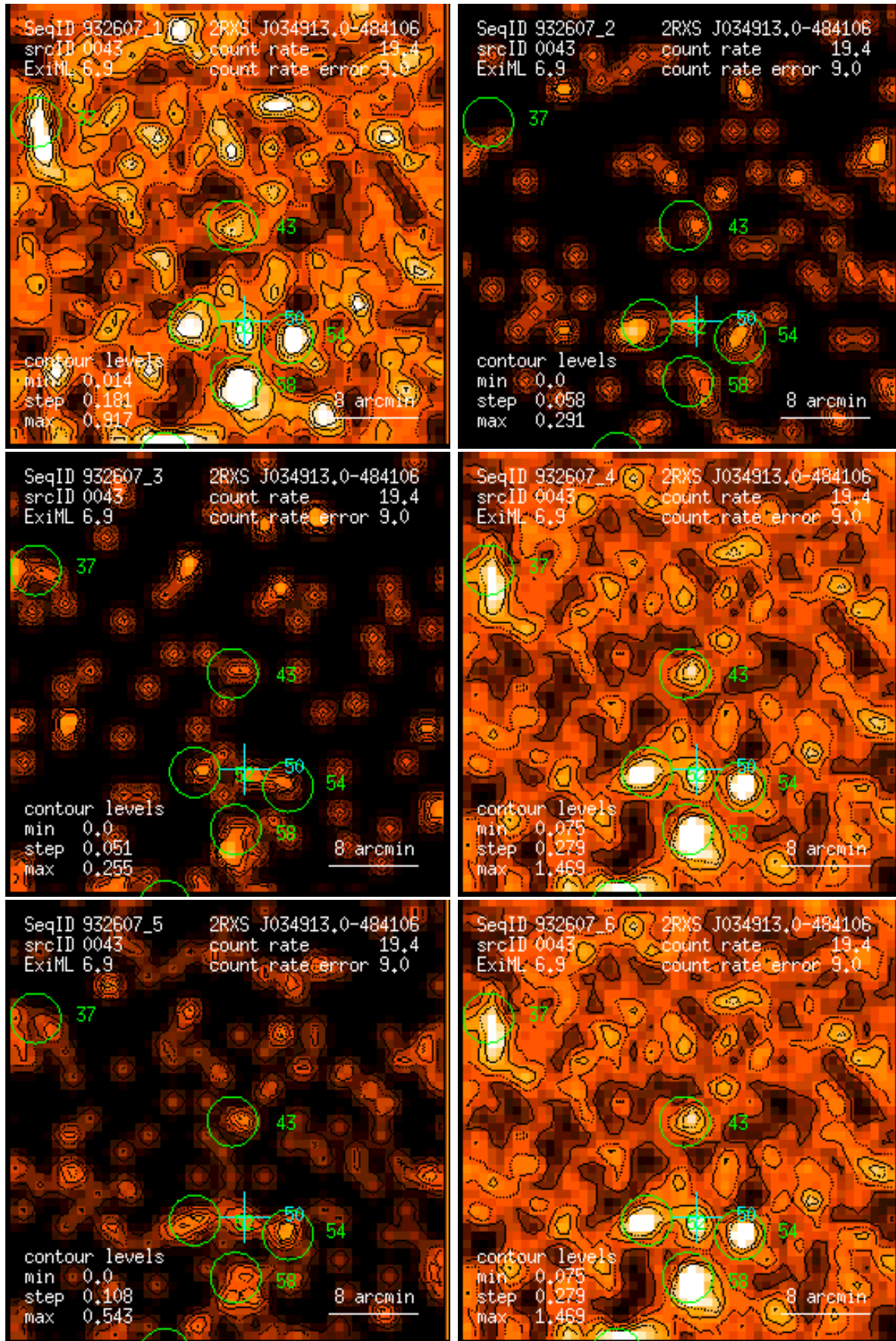
Figure 43: RASS 932607: detection 0043: band rate images, Gaussian filter: (1) PSPC channels 11 – 41, (2) 52 – 90, (3) 91 – 201, (4) 11 – 235, (5) 52 – 201, (6) 11 – 201. Broad band rates in counts/ks. Band rate contour levels in counts/ks/arcmin 2 .
