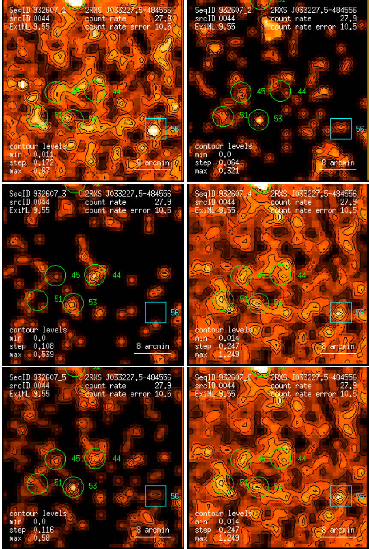
Figure 44: RASS 932607: detection 0044: band rate images, Gaussian filter: (1) PSPC channels 11 – 41, (2) 52 – 90, (3) 91 – 201, (4) 11 – 235, (5) 52 – 201, (6) 11 – 201. Broad band rates in counts/ks. Band rate contour levels in counts/ks/arcmin 2 .
