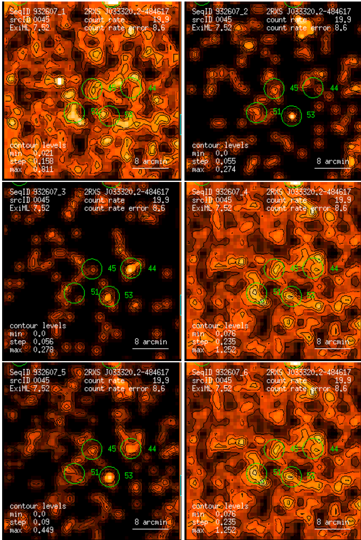
Figure 45: RASS 932607: detection 0045: band rate images, Gaussian filter: (1) PSPC channels 11 – 41, (2) 52 – 90, (3) 91 – 201, (4) 11 – 235, (5) 52 – 201, (6) 11 – 201. Broad band rates in counts/ks. Band rate contour levels in counts/ks/arcmin 2 .
