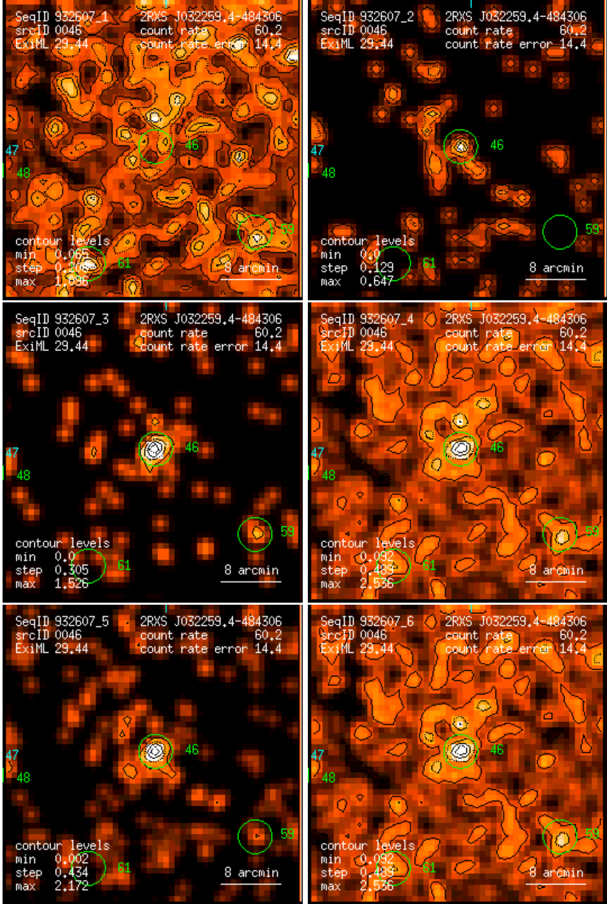
Figure 46: RASS 932607: detection 0046: band rate images, Gaussian filter: (1) PSPC channels 11 – 41, (2) 52 – 90, (3) 91 – 201, (4) 11 – 235, (5) 52 – 201, (6) 11 – 201. Broad band rates in counts/ks. Band rate contour levels in counts/ks/arcmin 2 .
