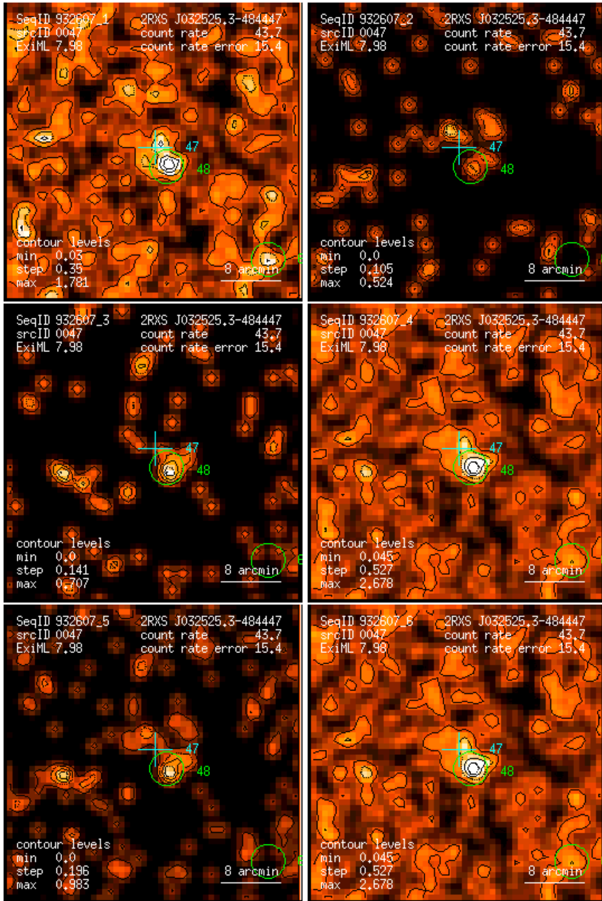
Figure 47: RASS 932607: detection 0047: band rate images, Gaussian filter: (1) PSPC channels 11 – 41, (2) 52 – 90, (3) 91 – 201, (4) 11 – 235, (5) 52 – 201, (6) 11 – 201. Broad band rates in counts/ks. Band rate contour levels in counts/ks/arcmin 2 .
