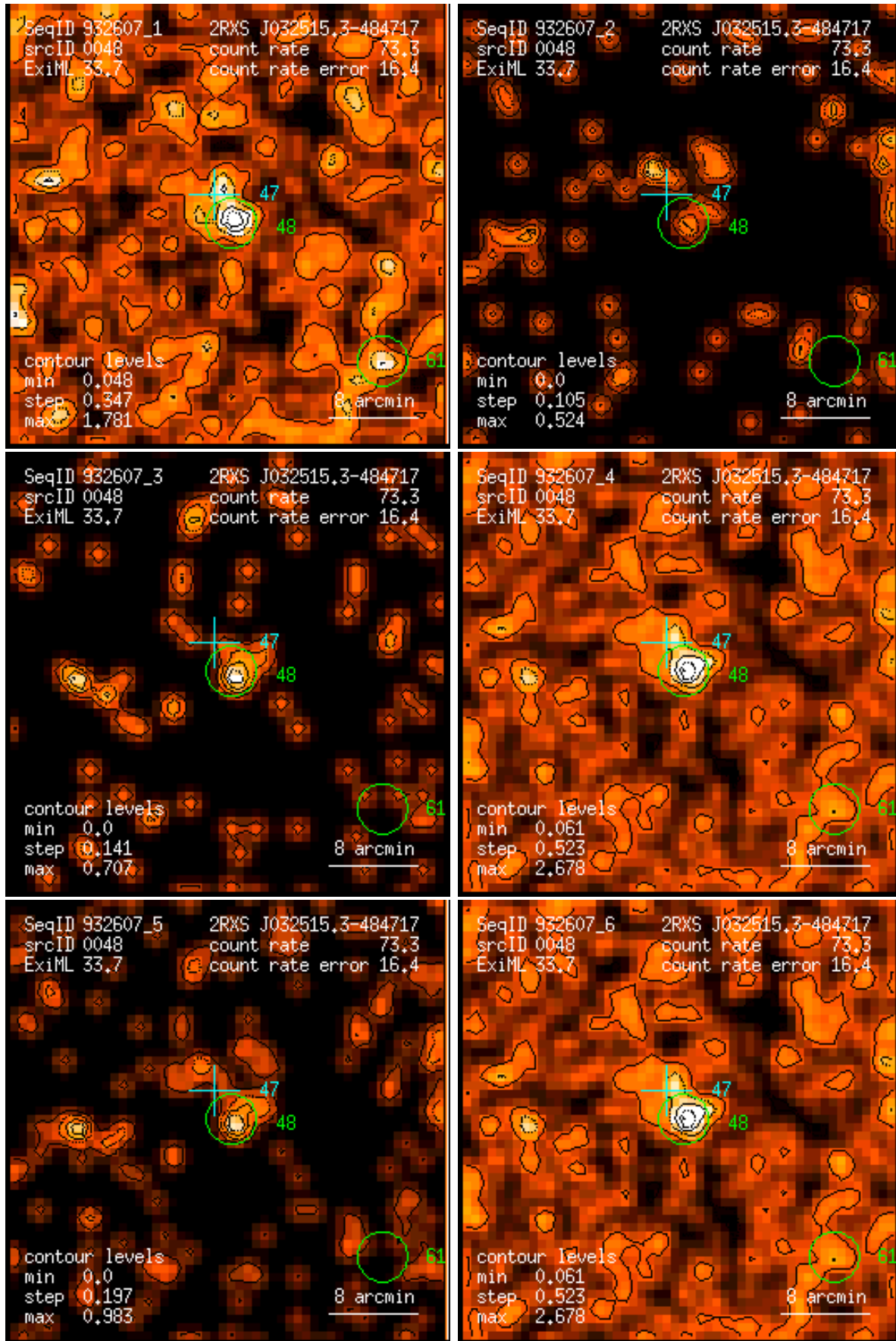
Figure 48: RASS 932607: detection 0048: band rate images, Gaussian filter: (1) PSPC channels 11 – 41, (2) 52 – 90, (3) 91 – 201, (4) 11 – 235, (5) 52 – 201, (6) 11 – 201. Broad band rates in counts/ks. Band rate contour levels in counts/ks/arcmin 2 .
