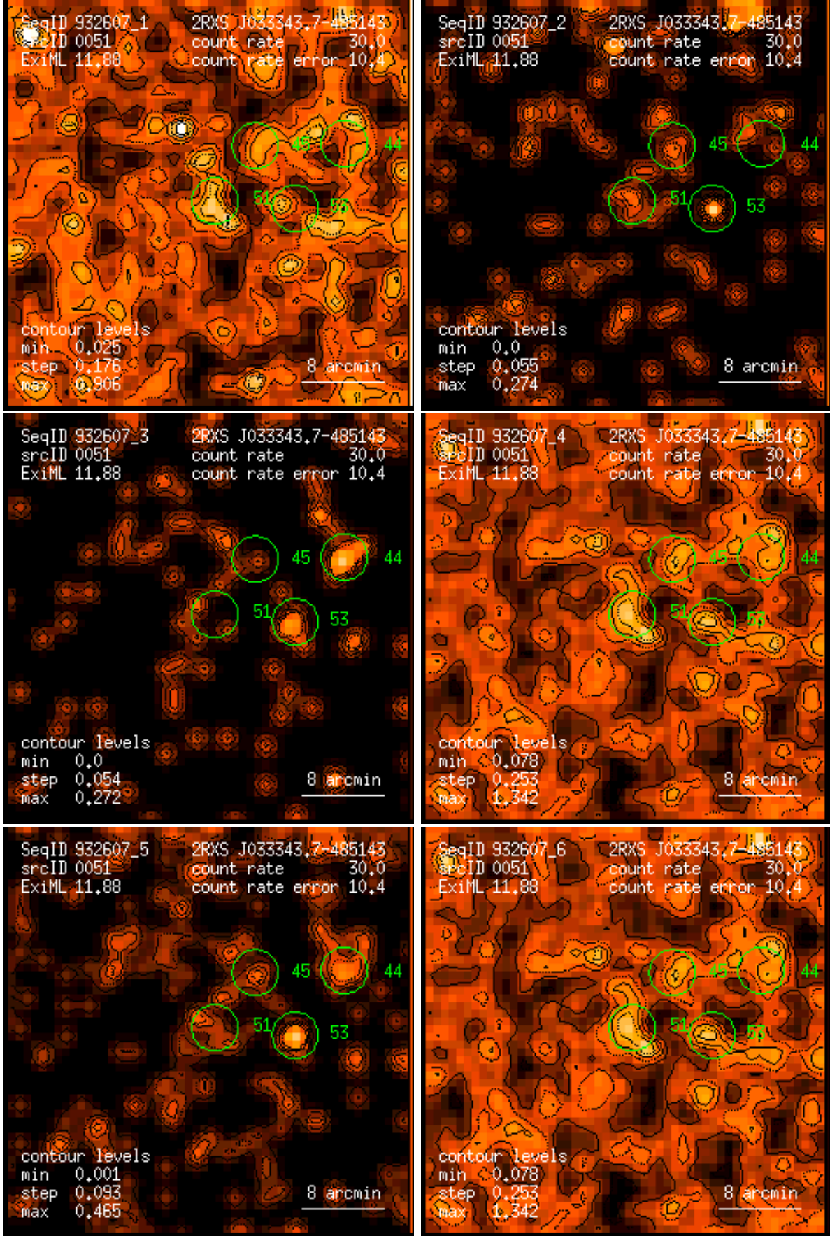
Figure 51: RASS 932607: detection 0051: band rate images, Gaussian filter: (1) PSPC channels 11 – 41, (2) 52 – 90, (3) 91 – 201, (4) 11 – 235, (5) 52 – 201, (6) 11 – 201. Broad band rates in counts/ks. Band rate contour levels in counts/ks/arcmin 2 .
