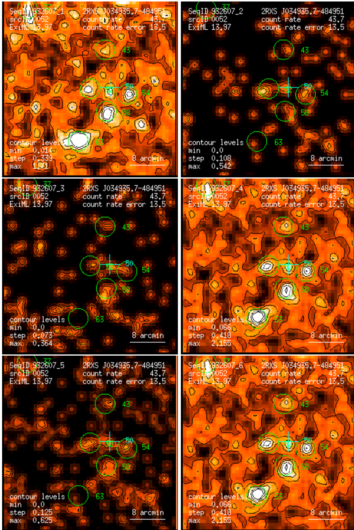
Figure 52: RASS 932607: detection 0052: band rate images, Gaussian filter: (1) PSPC channels 11 – 41, (2) 52 – 90, (3) 91 – 201, (4) 11 – 235, (5) 52 – 201, (6) 11 – 201. Broad band rates in counts/ks. Band rate contour levels in counts/ks/arcmin 2 .
