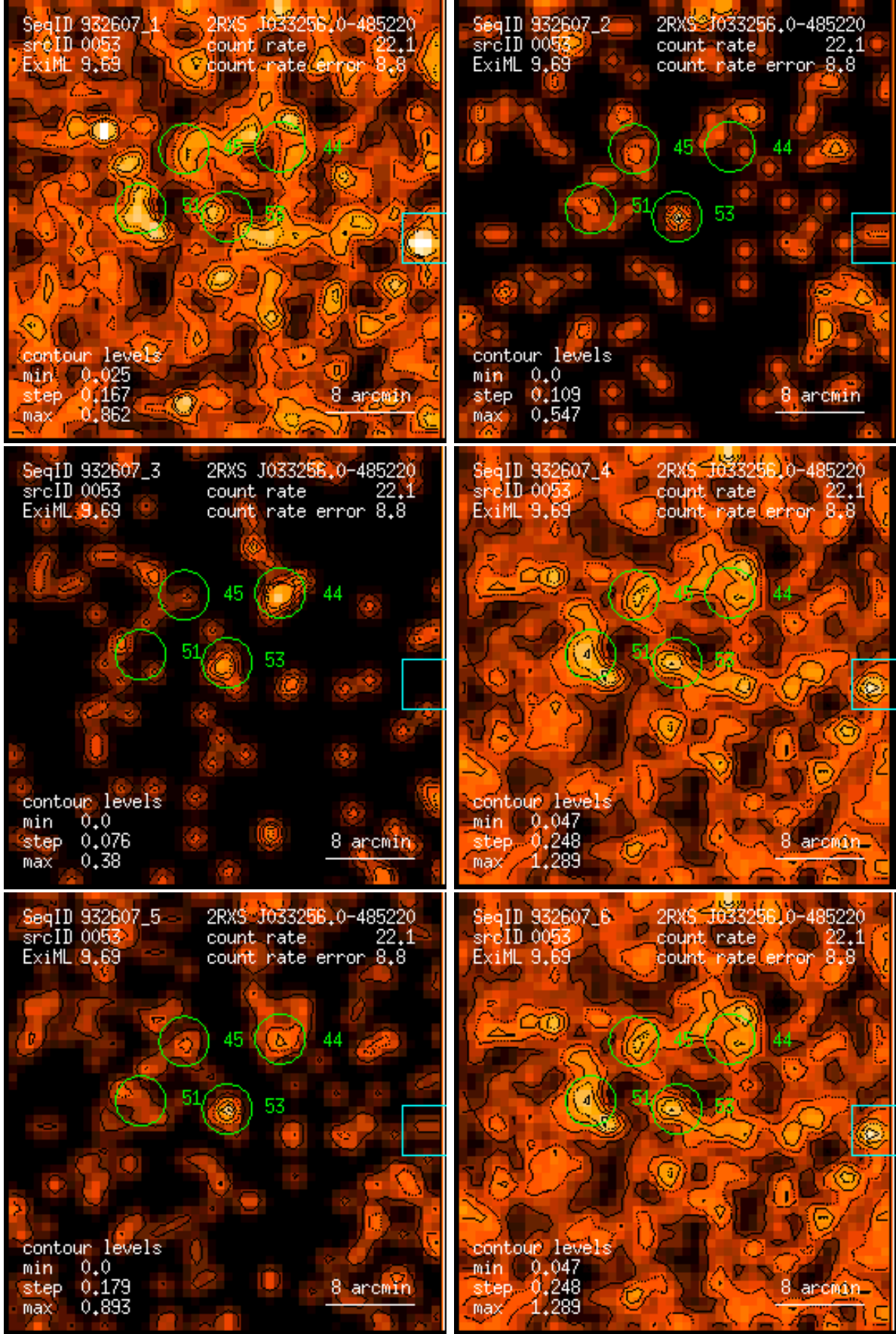
Figure 53: RASS 932607: detection 0053: band rate images, Gaussian filter: (1) PSPC channels 11 – 41, (2) 52 – 90, (3) 91 – 201, (4) 11 – 235, (5) 52 – 201, (6) 11 – 201. Broad band rates in counts/ks. Band rate contour levels in counts/ks/arcmin 2 .
