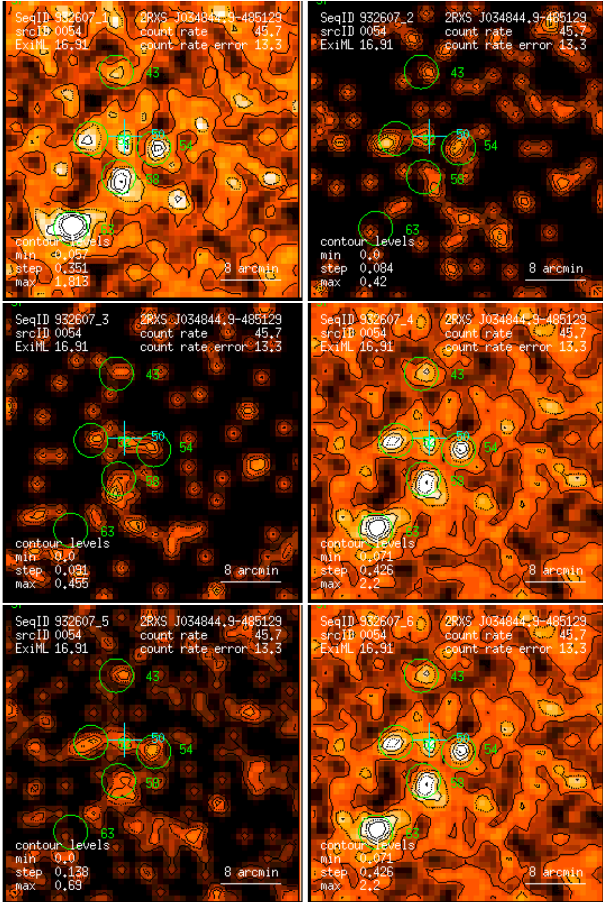
Figure 54: RASS 932607: detection 0054: band rate images, Gaussian filter: (1) PSPC channels 11 – 41, (2) 52 – 90, (3) 91 – 201, (4) 11 – 235, (5) 52 – 201, (6) 11 – 201. Broad band rates in counts/ks. Band rate contour levels in counts/ks/arcmin 2 .
