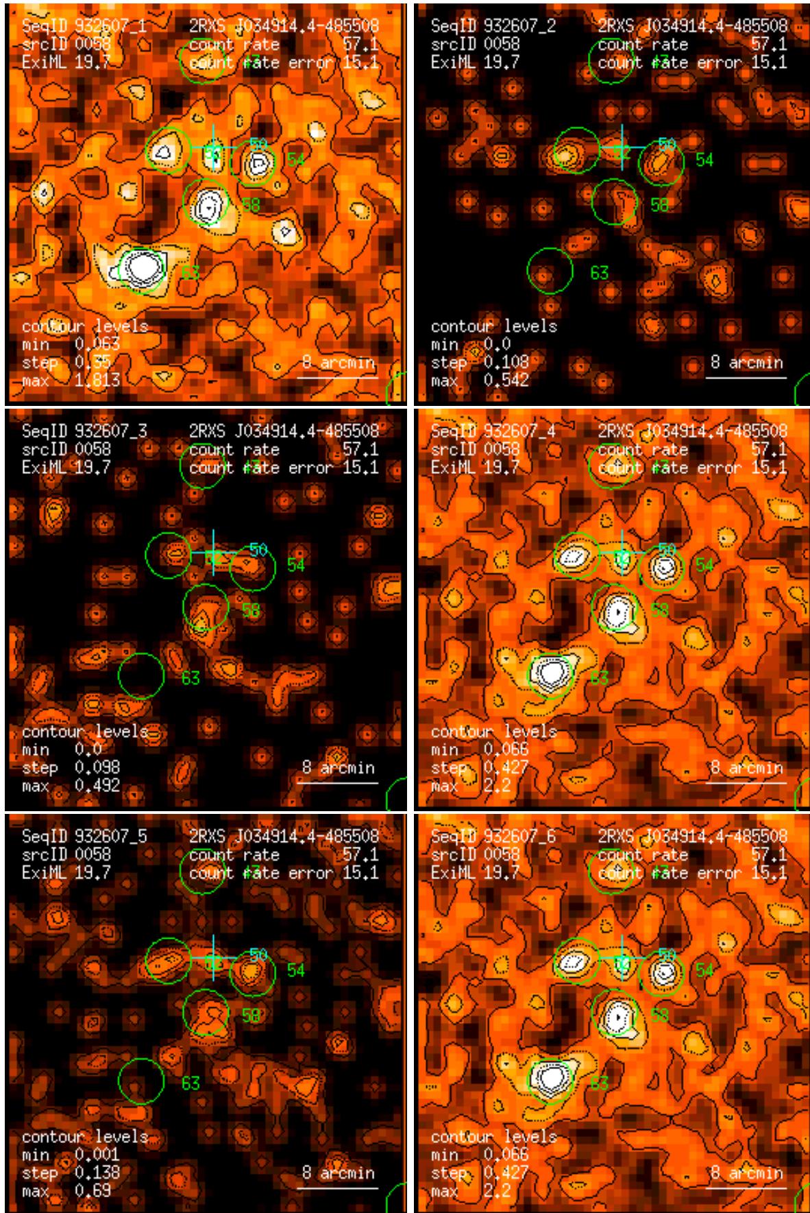
Figure 58: RASS 932607: detection 0058: band rate images, Gaussian filter: (1) PSPC channels 11 – 41, (2) 52 – 90, (3) 91 – 201, (4) 11 – 235, (5) 52 – 201, (6) 11 – 201. Broad band rates in counts/ks. Band rate contour levels in counts/ks/arcmin 2 .
