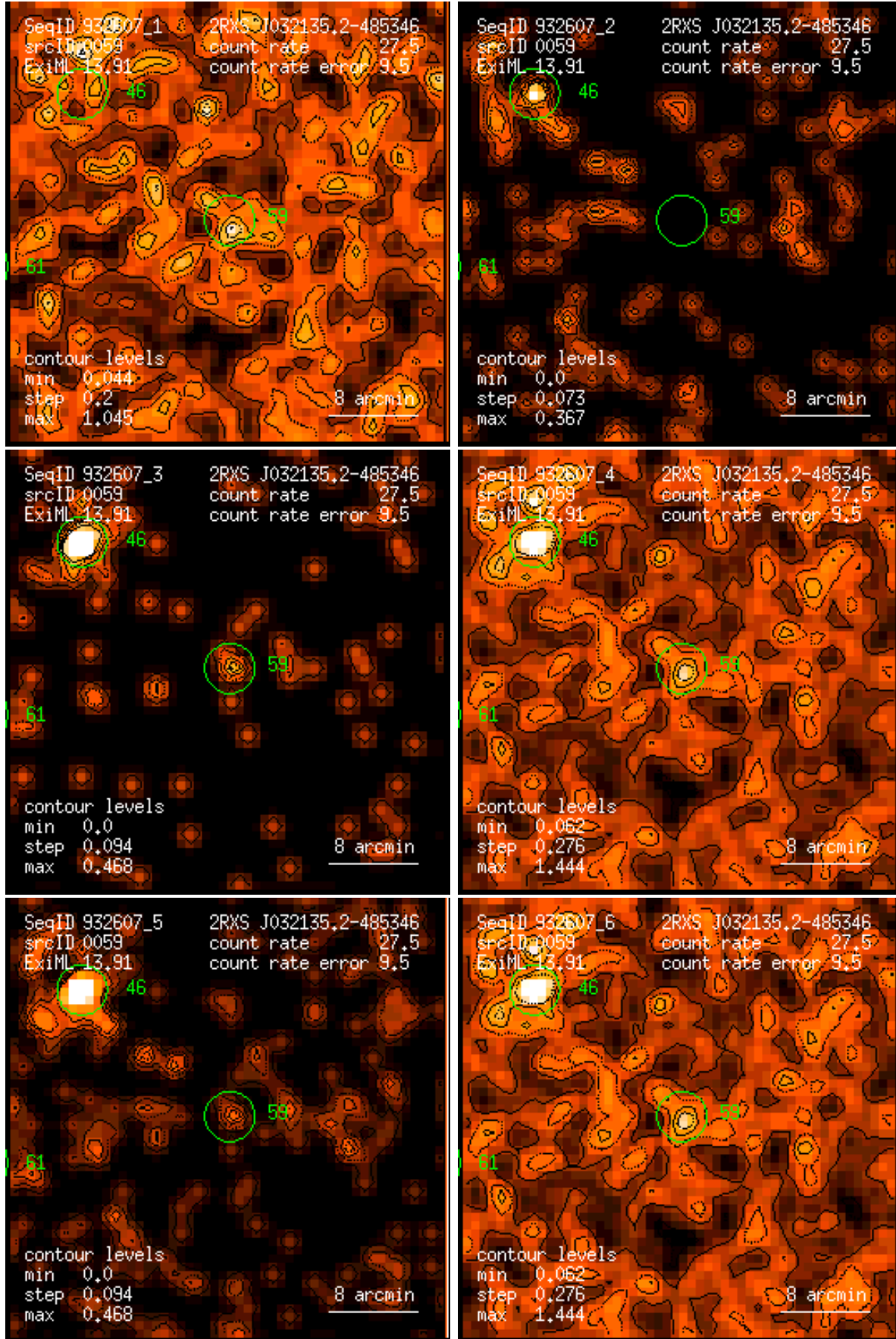
Figure 59: RASS 932607: detection 0059: band rate images, Gaussian filter: (1) PSPC channels 11 – 41, (2) 52 – 90, (3) 91 – 201, (4) 11 – 235, (5) 52 – 201, (6) 11 – 201. Broad band rates in counts/ks. Band rate contour levels in counts/ks/arcmin 2 .
