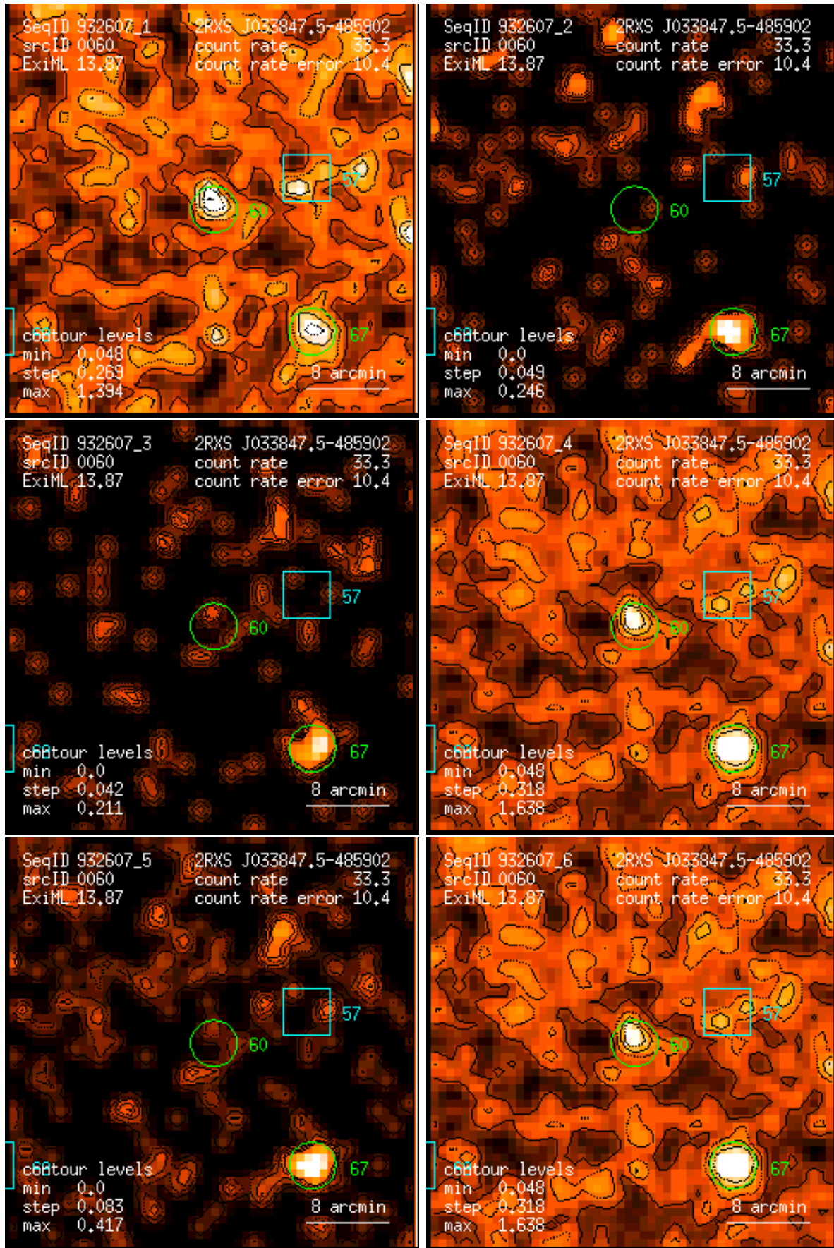
Figure 60: RASS 932607: detection 0060: band rate images, Gaussian filter: (1) PSPC channels 11 – 41, (2) 52 – 90, (3) 91 – 201, (4) 11 – 235, (5) 52 – 201, (6) 11 – 201. Broad band rates in counts/ks. Band rate contour levels in counts/ks/arcmin 2 .
