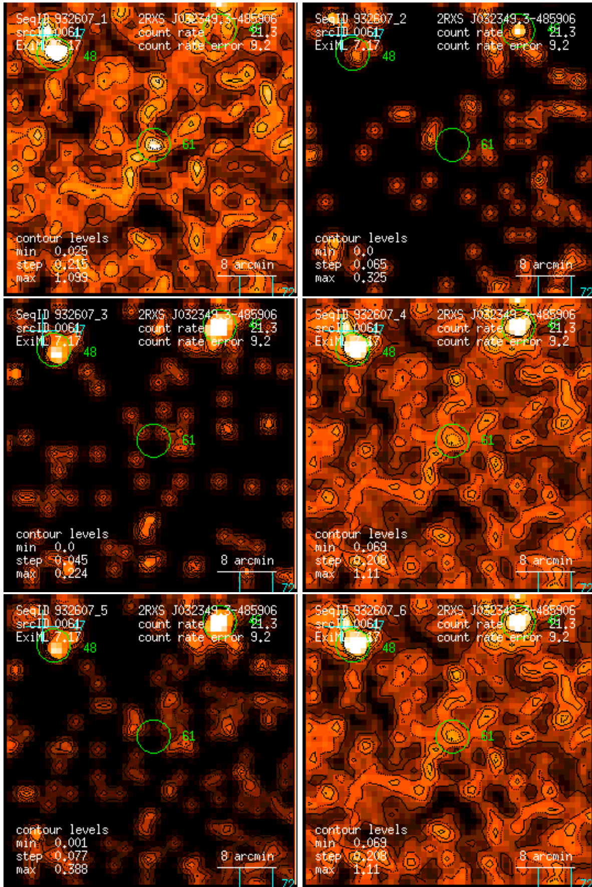
Figure 61: RASS 932607: detection 0061: band rate images, Gaussian filter: (1) PSPC channels 11 – 41, (2) 52 – 90, (3) 91 – 201, (4) 11 – 235, (5) 52 – 201, (6) 11 – 201. Broad band rates in counts/ks. Band rate contour levels in counts/ks/arcmin 2 .
