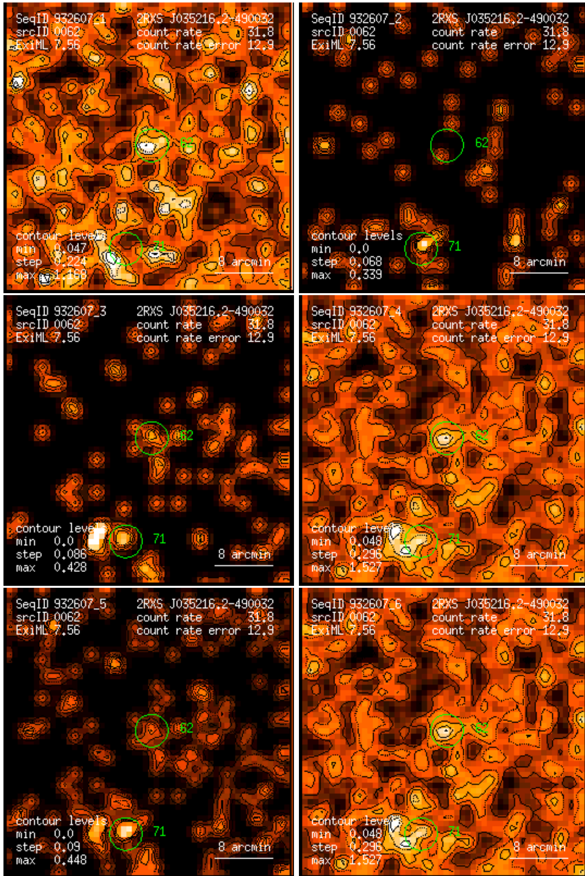
Figure 62: RASS 932607: detection 0062: band rate images, Gaussian filter: (1) PSPC channels 11 – 41, (2) 52 – 90, (3) 91 – 201, (4) 11 – 235, (5) 52 – 201, (6) 11 – 201. Broad band rates in counts/ks. Band rate contour levels in counts/ks/arcmin 2 .
