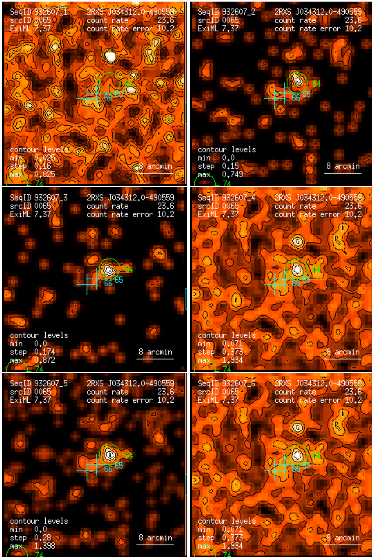
Figure 65: RASS 932607: detection 0065: band rate images, Gaussian filter: (1) PSPC channels 11 – 41, (2) 52 – 90, (3) 91 – 201, (4) 11 – 235, (5) 52 – 201, (6) 11 – 201. Broad band rates in counts/ks. Band rate contour levels in counts/ks/arcmin 2 .
