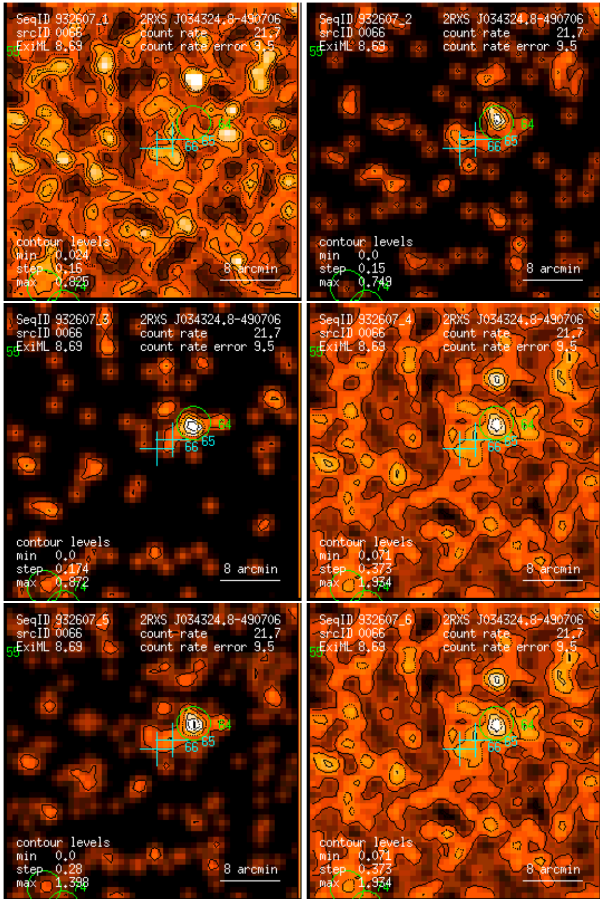
Figure 66: RASS 932607: detection 0066: band rate images, Gaussian filter: (1) PSPC channels 11 – 41, (2) 52 – 90, (3) 91 – 201, (4) 11 – 235, (5) 52 – 201, (6) 11 – 201. Broad band rates in counts/ks. Band rate contour levels in counts/ks/arcmin 2 .
