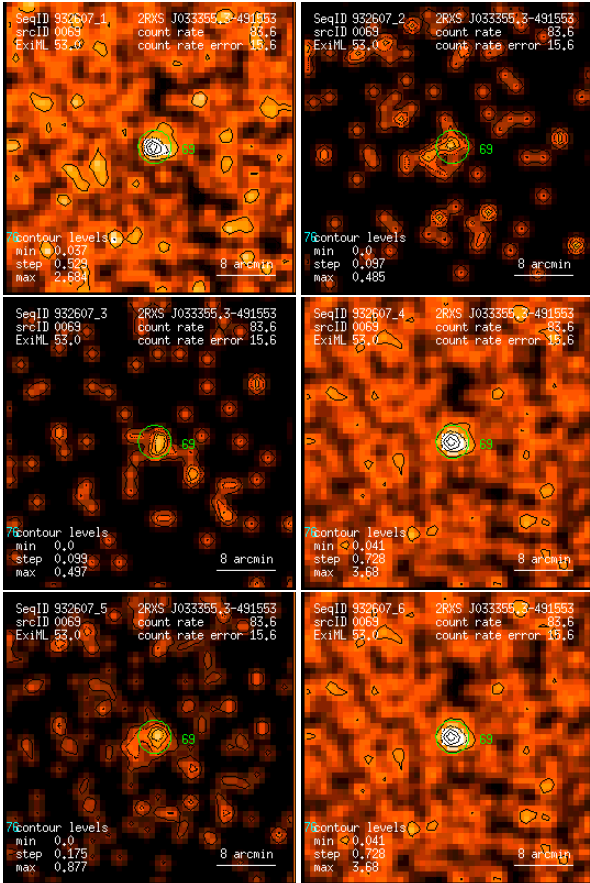
Figure 69: RASS 932607: detection 0069: band rate images, Gaussian filter: (1) PSPC channels 11 – 41, (2) 52 – 90, (3) 91 – 201, (4) 11 – 235, (5) 52 – 201, (6) 11 – 201. Broad band rates in counts/ks. Band rate contour levels in counts/ks/arcmin 2 .
