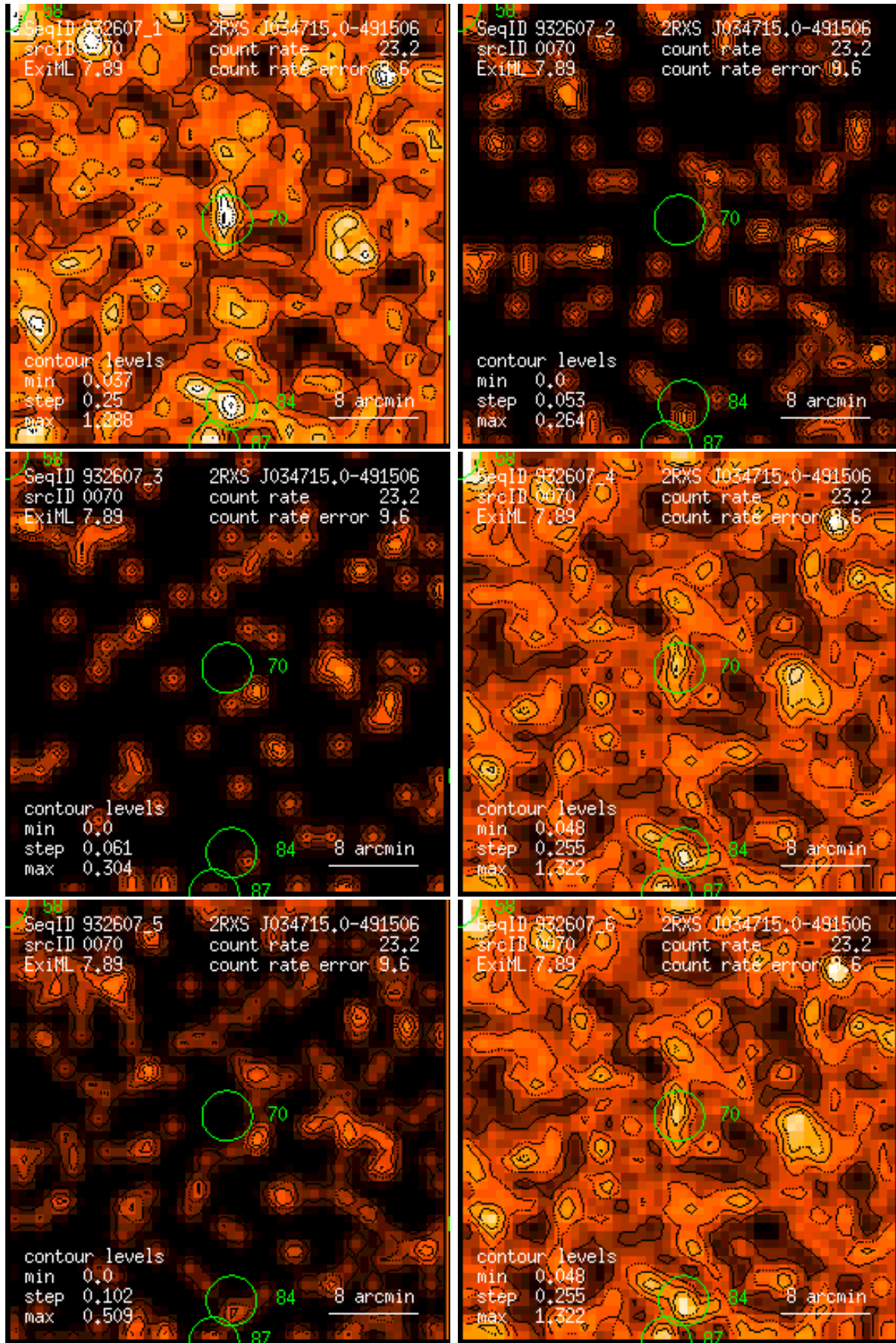
Figure 70: RASS 932607: detection 0070: band rate images, Gaussian filter: (1) PSPC channels 11 – 41, (2) 52 – 90, (3) 91 – 201, (4) 11 – 235, (5) 52 – 201, (6) 11 – 201. Broad band rates in counts/ks. Band rate contour levels in counts/ks/arcmin 2 .
