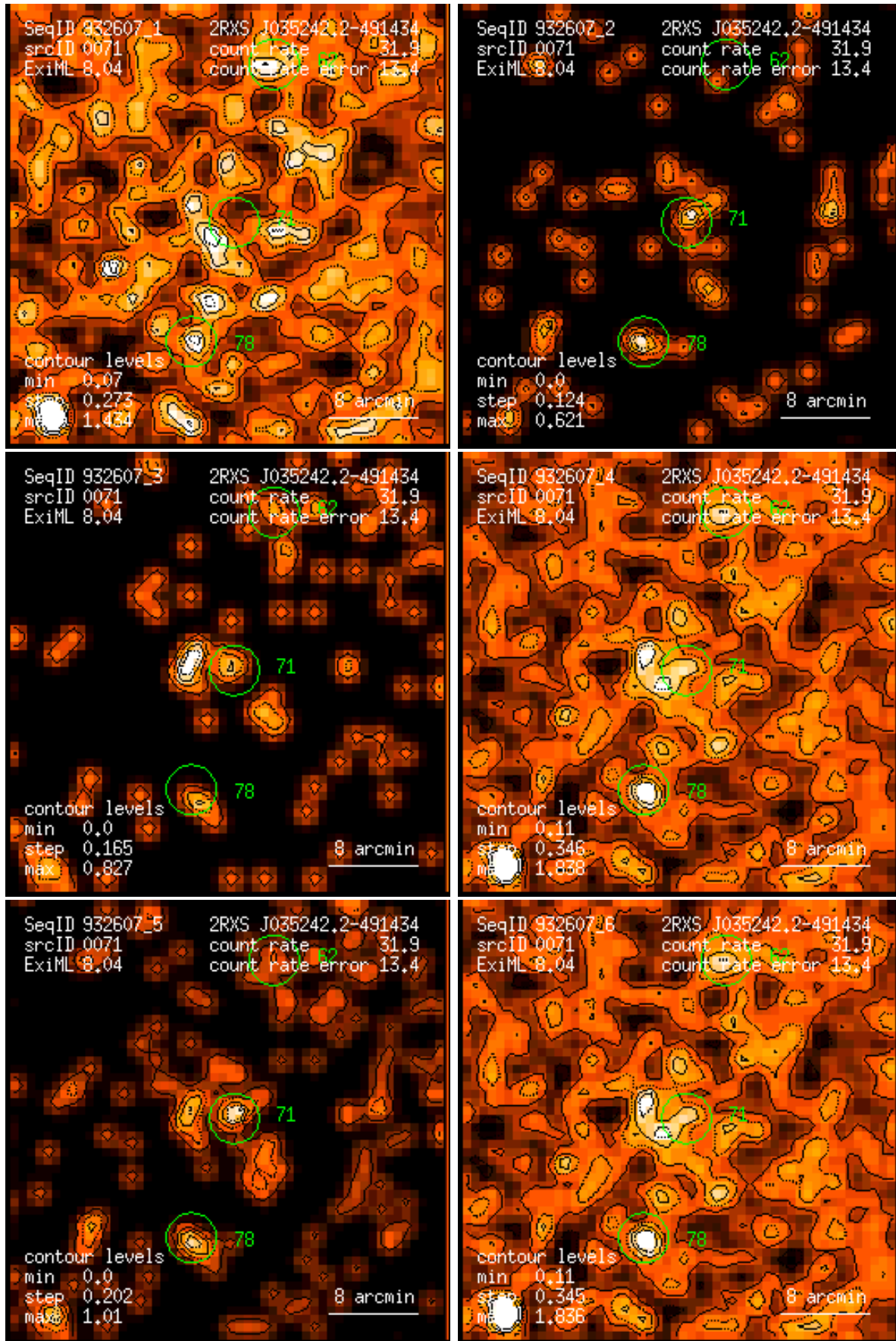
Figure 71: RASS 932607: detection 0071: band rate images, Gaussian filter: (1) PSPC channels 11 – 41, (2) 52 – 90, (3) 91 – 201, (4) 11 – 235, (5) 52 – 201, (6) 11 – 201. Broad band rates in counts/ks. Band rate contour levels in counts/ks/arcmin 2 .
