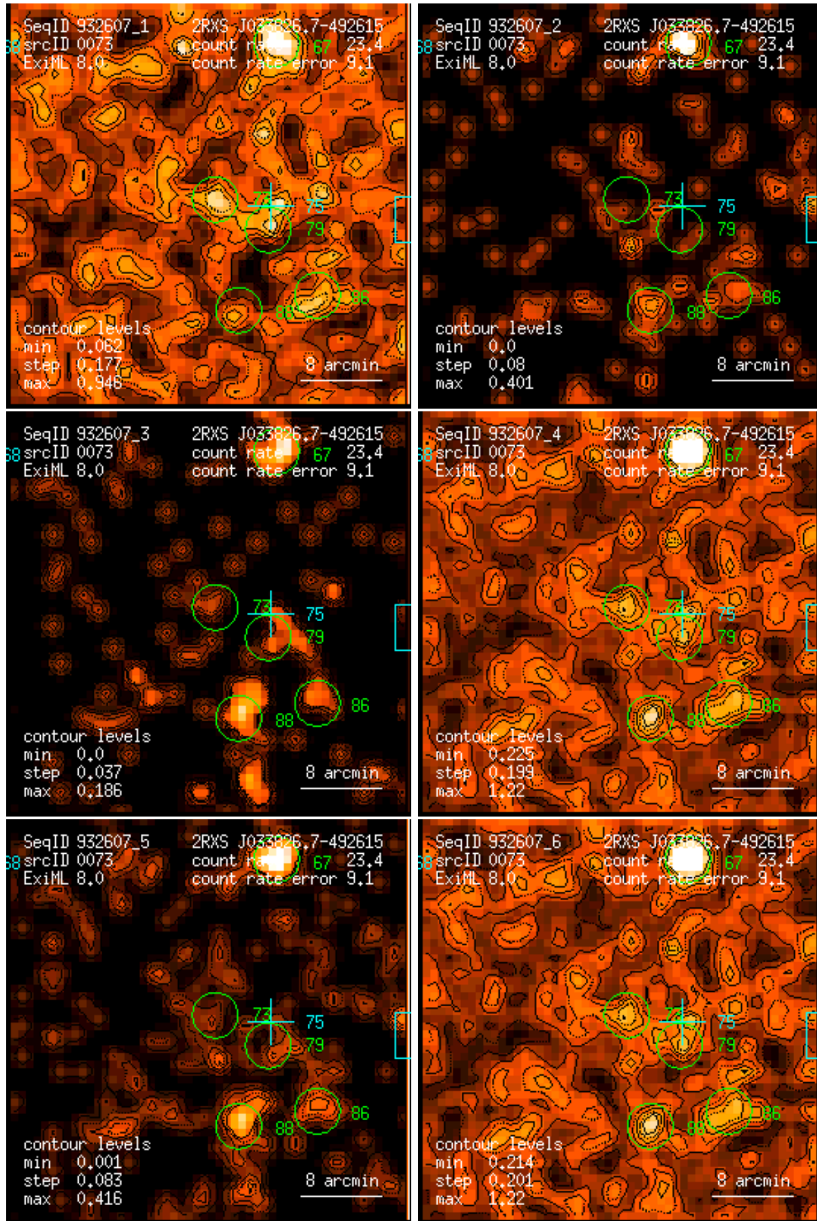
Figure 73: RASS 932607: detection 0073: band rate images, Gaussian filter: (1) PSPC channels 11 – 41, (2) 52 – 90, (3) 91 – 201, (4) 11 – 235, (5) 52 – 201, (6) 11 – 201. Broad band rates in counts/ks. Band rate contour levels in counts/ks/arcmin 2 .
