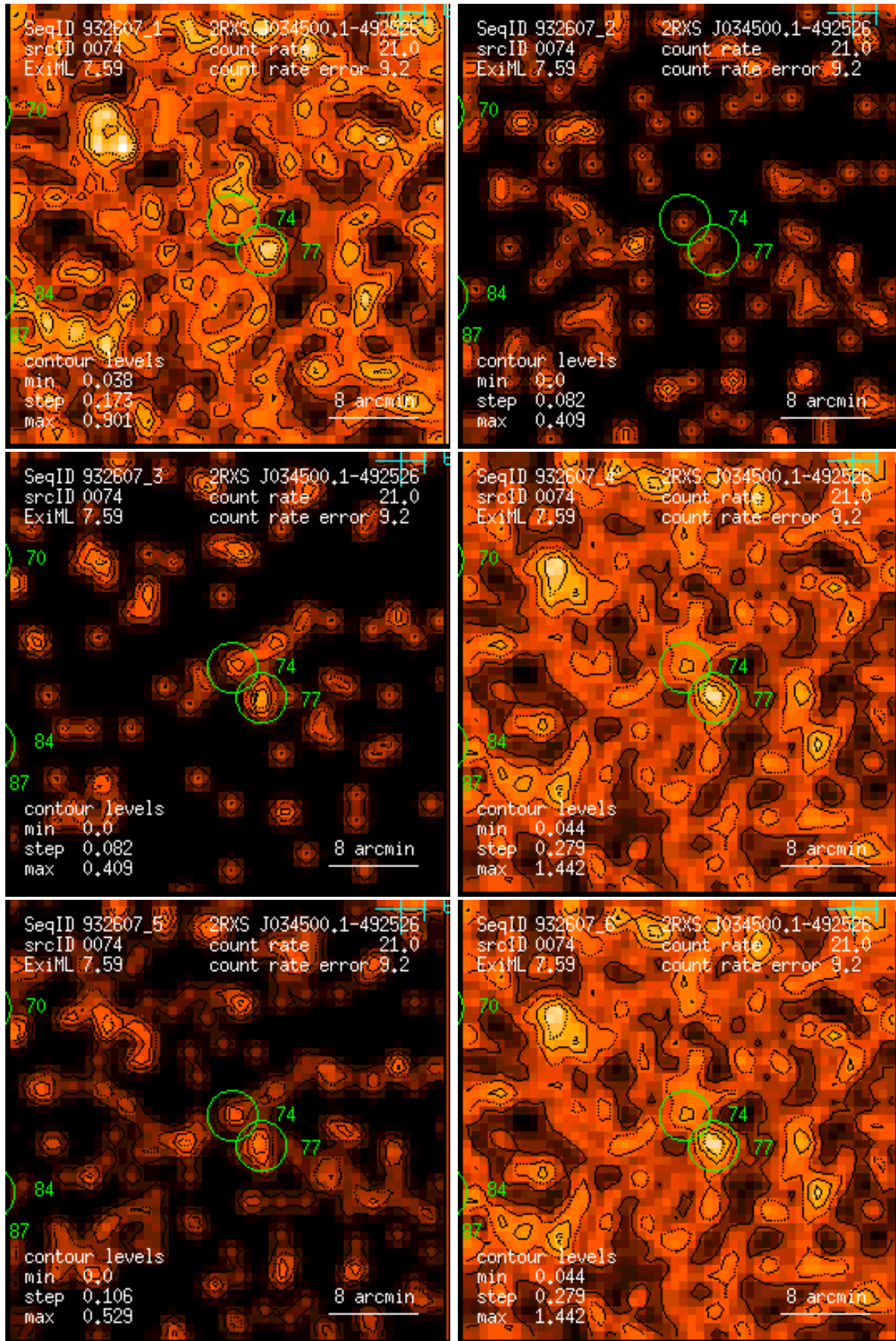
Figure 74: RASS 932607: detection 0074: band rate images, Gaussian filter: (1) PSPC channels 11 – 41, (2) 52 – 90, (3) 91 – 201, (4) 11 – 235, (5) 52 – 201, (6) 11 – 201. Broad band rates in counts/ks. Band rate contour levels in counts/ks/arcmin 2 .
