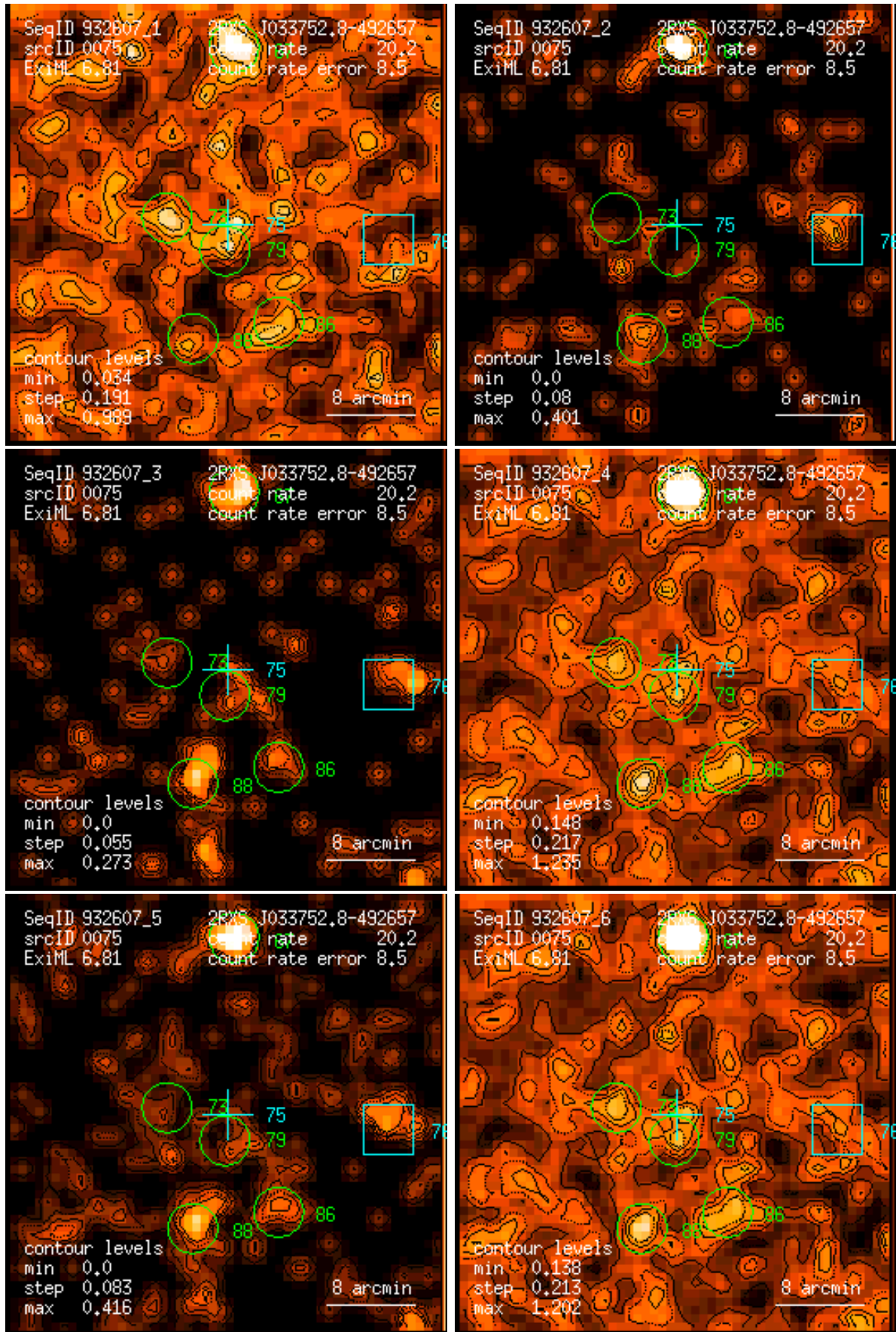
Figure 75: RASS 932607: detection 0075: band rate images, Gaussian filter: (1) PSPC channels 11 – 41, (2) 52 – 90, (3) 91 – 201, (4) 11 – 235, (5) 52 – 201, (6) 11 – 201. Broad band rates in counts/ks. Band rate contour levels in counts/ks/arcmin 2 .
