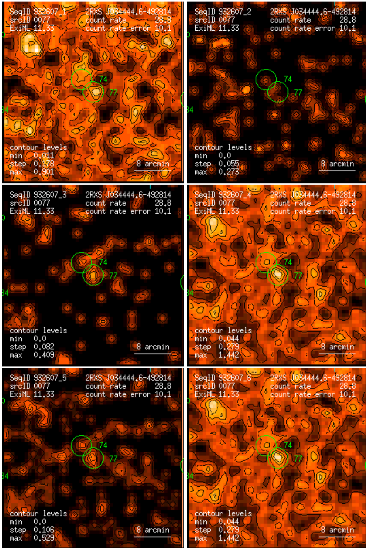
Figure 77: RASS 932607: detection 0077: band rate images, Gaussian filter: (1) PSPC channels 11 – 41, (2) 52 – 90, (3) 91 – 201, (4) 11 – 235, (5) 52 – 201, (6) 11 – 201. Broad band rates in counts/ks. Band rate contour levels in counts/ks/arcmin 2 .
