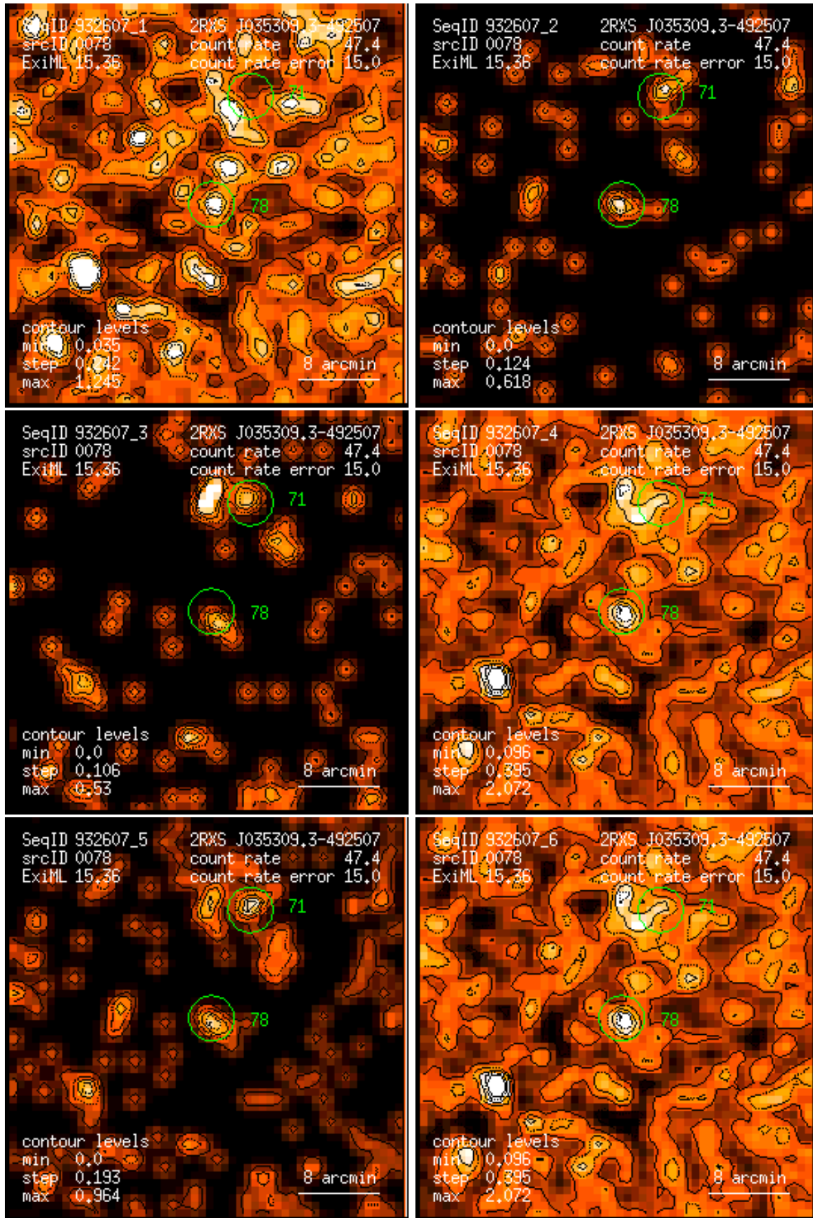
Figure 78: RASS 932607: detection 0078: band rate images, Gaussian filter: (1) PSPC channels 11 – 41, (2) 52 – 90, (3) 91 – 201, (4) 11 – 235, (5) 52 – 201, (6) 11 – 201. Broad band rates in counts/ks. Band rate contour levels in counts/ks/arcmin 2 .
