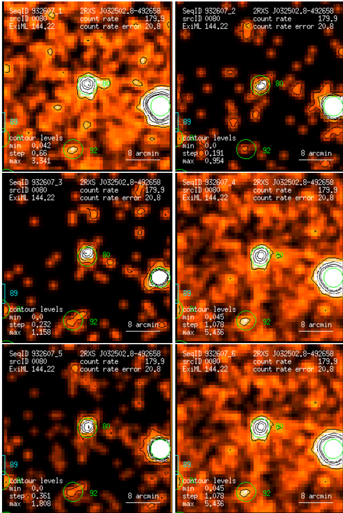
Figure 80: RASS 932607: detection 0080: band rate images, Gaussian filter: (1) PSPC channels 11 – 41, (2) 52 – 90, (3) 91 – 201, (4) 11 – 235, (5) 52 – 201, (6) 11 – 201. Broad band rates in counts/ks. Band rate contour levels in counts/ks/arcmin 2 .
