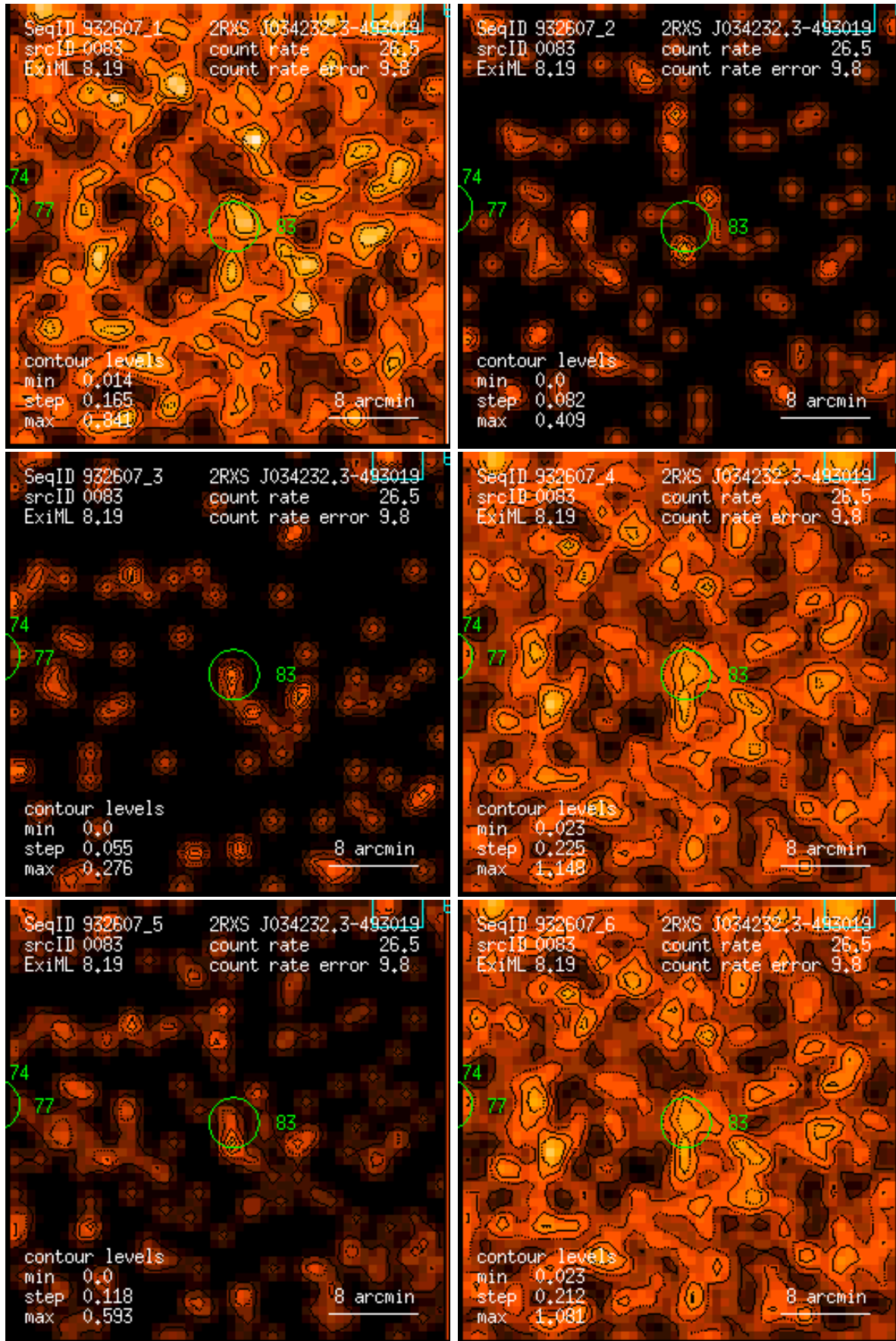
Figure 83: RASS 932607: detection 0083: band rate images, Gaussian filter: (1) PSPC channels 11 – 41, (2) 52 – 90, (3) 91 – 201, (4) 11 – 235, (5) 52 – 201, (6) 11 – 201. Broad band rates in counts/ks. Band rate contour levels in counts/ks/arcmin 2 .
