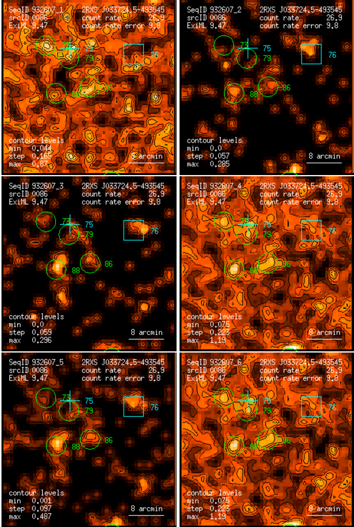
Figure 86: RASS 932607: detection 0086: band rate images, Gaussian filter: (1) PSPC channels 11 – 41, (2) 52 – 90, (3) 91 – 201, (4) 11 – 235, (5) 52 – 201, (6) 11 – 201. Broad band rates in counts/ks. Band rate contour levels in counts/ks/arcmin 2 .
