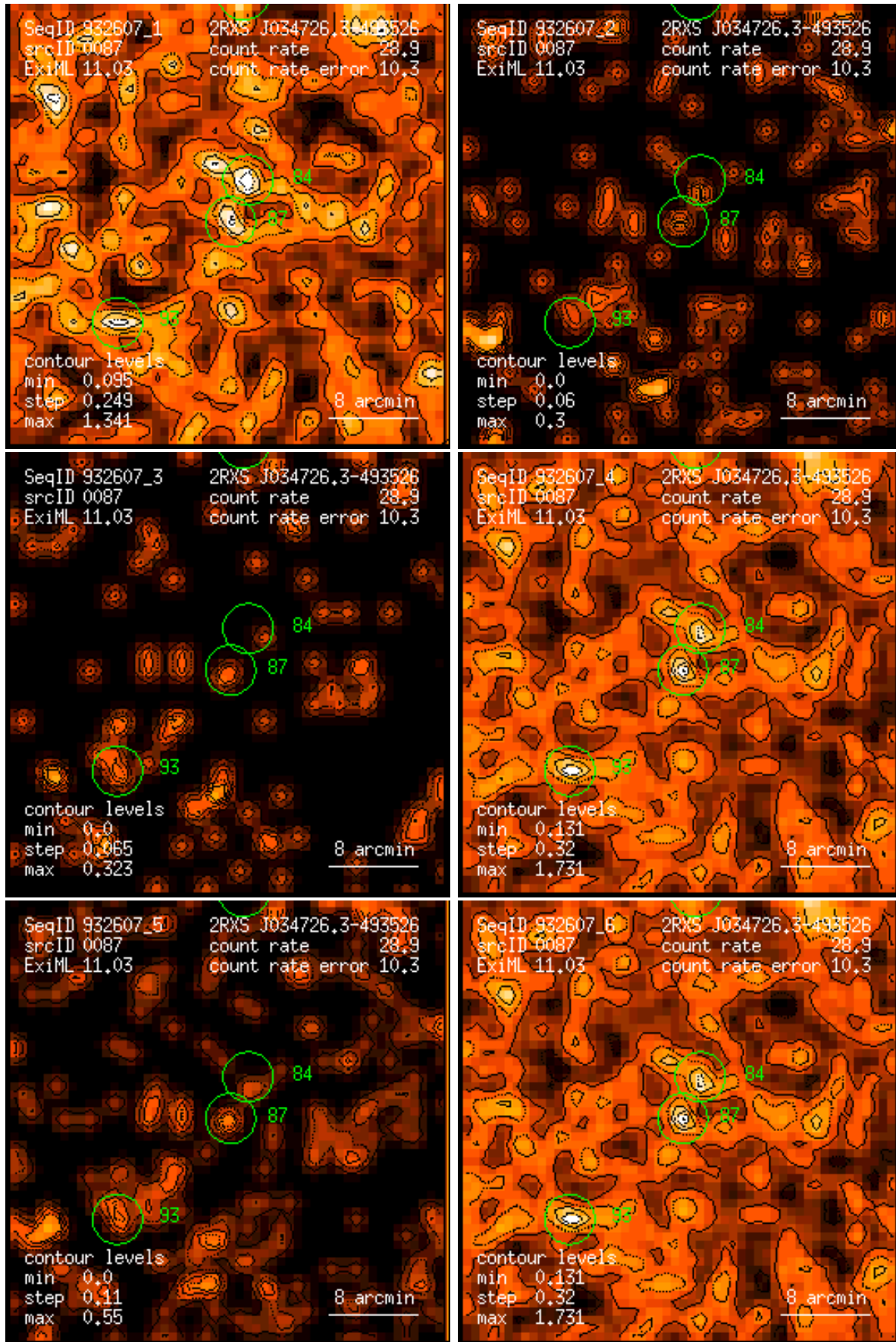
Figure 87: RASS 932607: detection 0087: band rate images, Gaussian filter: (1) PSPC channels 11 – 41, (2) 52 – 90, (3) 91 – 201, (4) 11 – 235, (5) 52 – 201, (6) 11 – 201. Broad band rates in counts/ks. Band rate contour levels in counts/ks/arcmin 2 .
