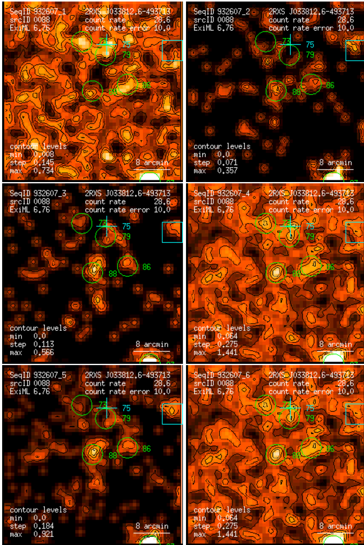
Figure 88: RASS 932607: detection 0088: band rate images, Gaussian filter: (1) PSPC channels 11 – 41, (2) 52 – 90, (3) 91 – 201, (4) 11 – 235, (5) 52 – 201, (6) 11 – 201. Broad band rates in counts/ks. Band rate contour levels in counts/ks/arcmin 2 .
