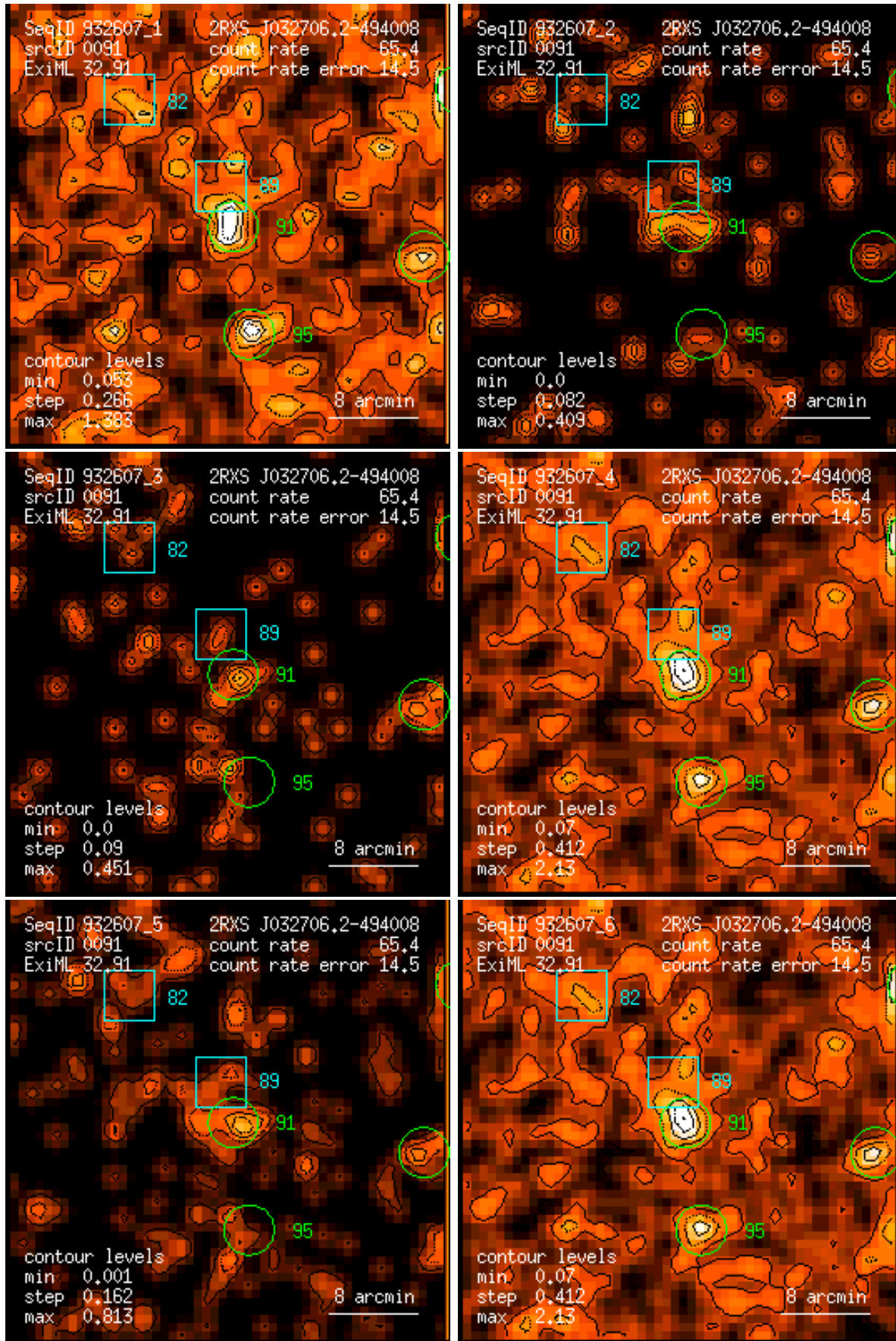
Figure 91: RASS 932607: detection 0091: band rate images, Gaussian filter: (1) PSPC channels 11 – 41, (2) 52 – 90, (3) 91 – 201, (4) 11 – 235, (5) 52 – 201, (6) 11 – 201. Broad band rates in counts/ks. Band rate contour levels in counts/ks/arcmin 2 .
