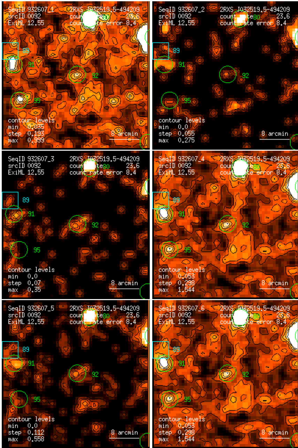
Figure 92: RASS 932607: detection 0092: band rate images, Gaussian filter: (1) PSPC channels 11 – 41, (2) 52 – 90, (3) 91 – 201, (4) 11 – 235, (5) 52 – 201, (6) 11 – 201. Broad band rates in counts/ks. Band rate contour levels in counts/ks/arcmin 2 .
