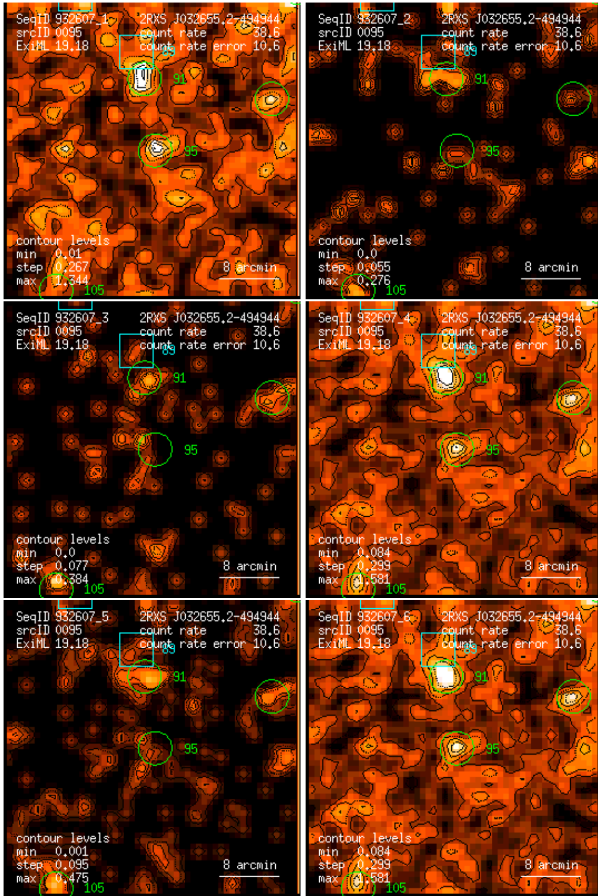
Figure 95: RASS 932607: detection 0095: band rate images, Gaussian filter: (1) PSPC channels 11 – 41, (2) 52 – 90, (3) 91 – 201, (4) 11 – 235, (5) 52 – 201, (6) 11 – 201. Broad band rates in counts/ks. Band rate contour levels in counts/ks/arcmin 2 .
