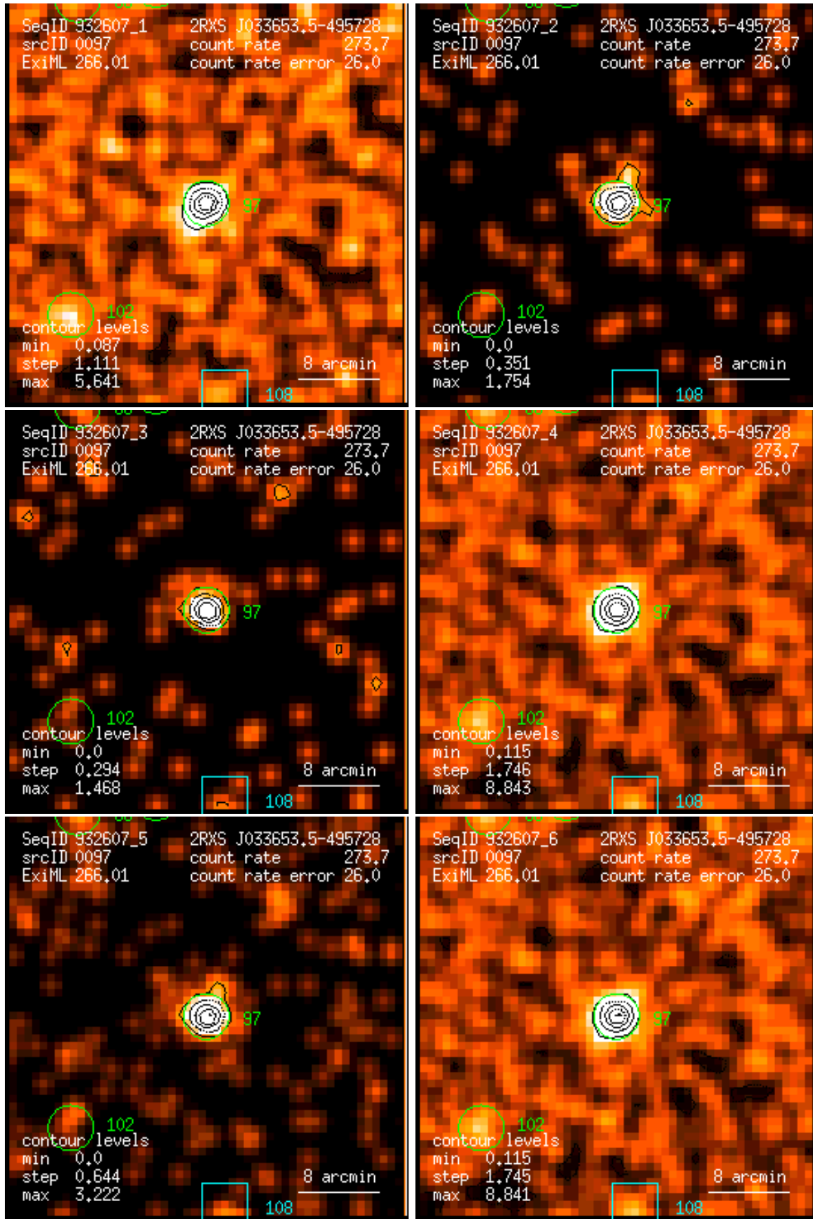
Figure 97: RASS 932607: detection 0097: band rate images, Gaussian filter: (1) PSPC channels 11 – 41, (2) 52 – 90, (3) 91 – 201, (4) 11 – 235, (5) 52 – 201, (6) 11 – 201. Broad band rates in counts/ks. Band rate contour levels in counts/ks/arcmin 2 .
