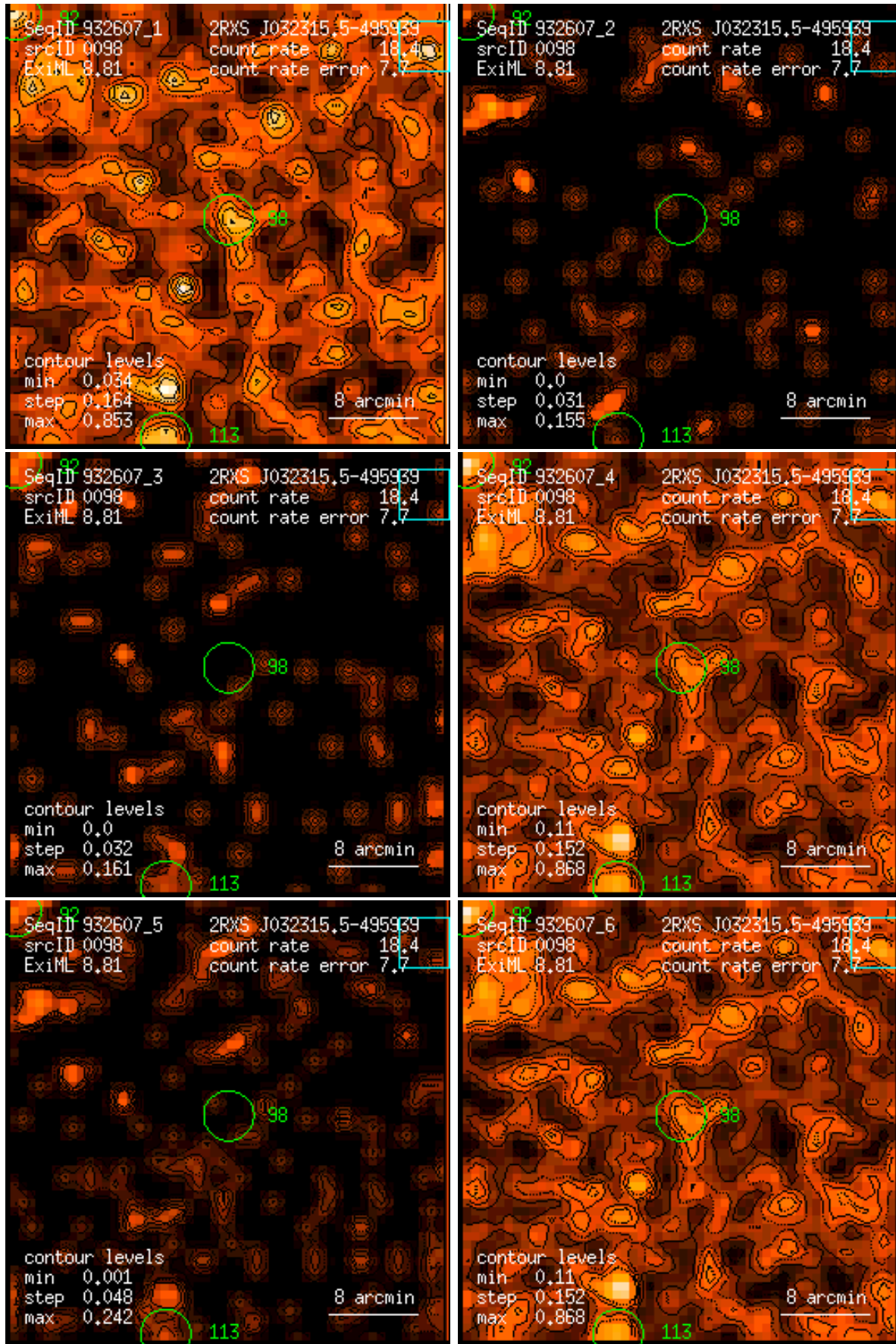
Figure 98: RASS 932607: detection 0098: band rate images, Gaussian filter: (1) PSPC channels 11 – 41, (2) 52 – 90, (3) 91 – 201, (4) 11 – 235, (5) 52 – 201, (6) 11 – 201. Broad band rates in counts/ks. Band rate contour levels in counts/ks/arcmin 2 .
