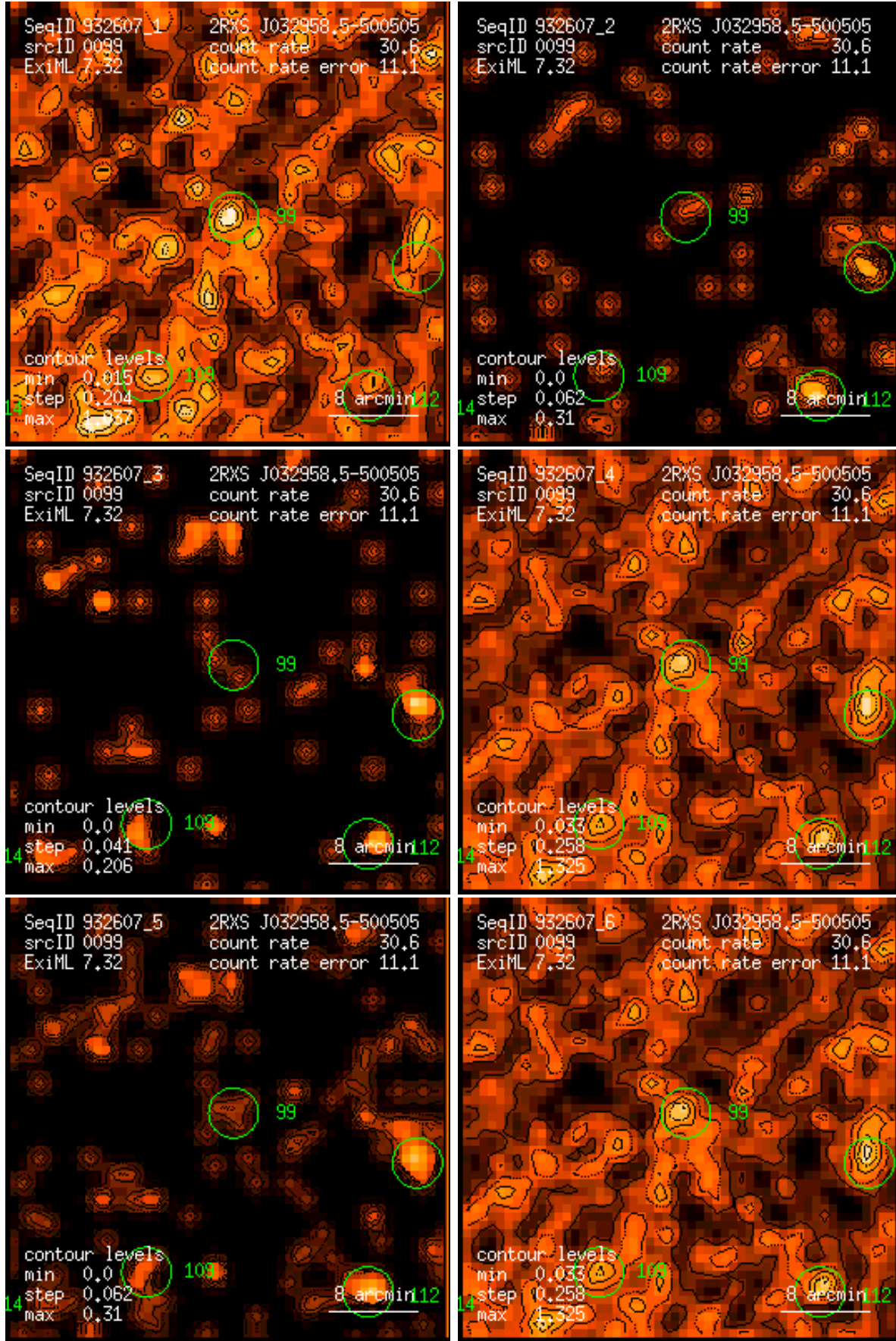
Figure 99: RASS 932607: detection 0099: band rate images, Gaussian filter: (1) PSPC channels 11 – 41, (2) 52 – 90, (3) 91 – 201, (4) 11 – 235, (5) 52 – 201, (6) 11 – 201. Broad band rates in counts/ks. Band rate contour levels in counts/ks/arcmin 2 .
