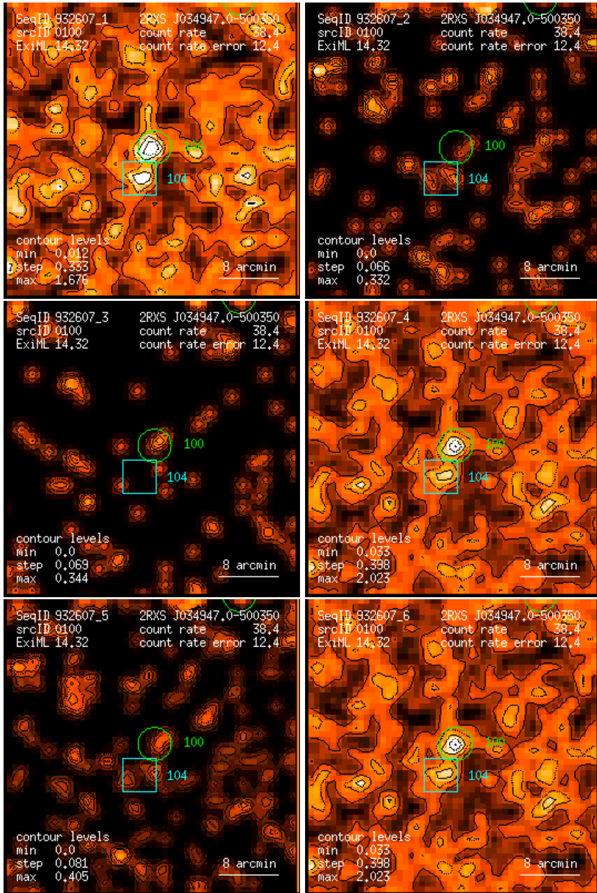
Figure 100: RASS 932607: detection 0100: band rate images, Gaussian filter: (1) PSPC channels 11 – 41, (2) 52 – 90, (3) 91 – 201, (4) 11 – 235, (5) 52 – 201, (6) 11 – 201. Broad band rates in counts/ks. Band rate contour levels in counts/ks/arcmin 2 .
