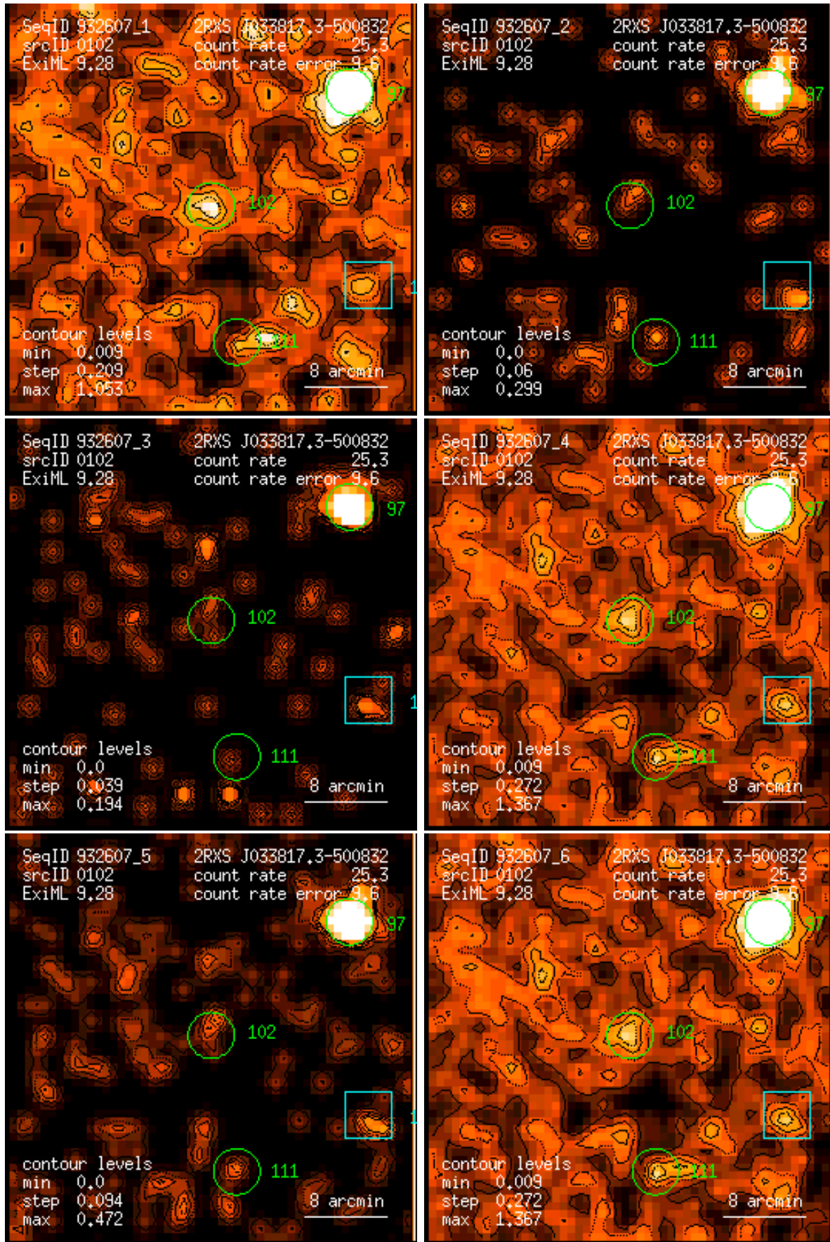
Figure 102: RASS 932607: detection 0102: band rate images, Gaussian filter: (1) PSPC channels 11 – 41, (2) 52 – 90, (3) 91 – 201, (4) 11 – 235, (5) 52 – 201, (6) 11 – 201. Broad band rates in counts/ks. Band rate contour levels in counts/ks/arcmin 2 .
