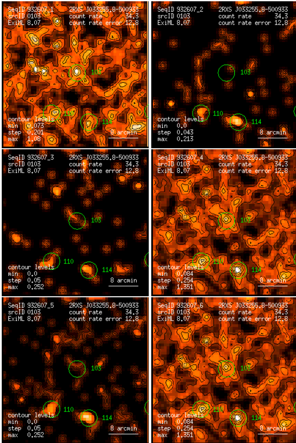
Figure 103: RASS 932607: detection 0103: band rate images, Gaussian filter: (1) PSPC channels 11 – 41, (2) 52 – 90, (3) 91 – 201, (4) 11 – 235, (5) 52 – 201, (6) 11 – 201. Broad band rates in counts/ks. Band rate contour levels in counts/ks/arcmin 2 .
