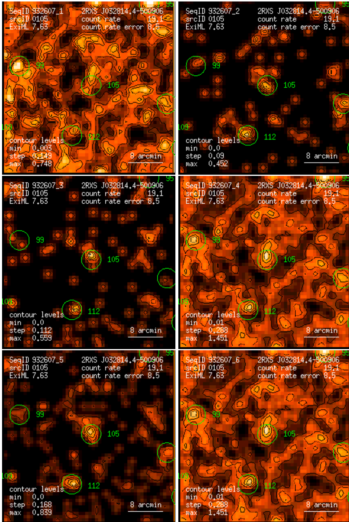
Figure 105: RASS 932607: detection 0105: band rate images, Gaussian filter: (1) PSPC channels 11 – 41, (2) 52 – 90, (3) 91 – 201, (4) 11 – 235, (5) 52 – 201, (6) 11 – 201. Broad band rates in counts/ks. Band rate contour levels in counts/ks/arcmin 2 .
