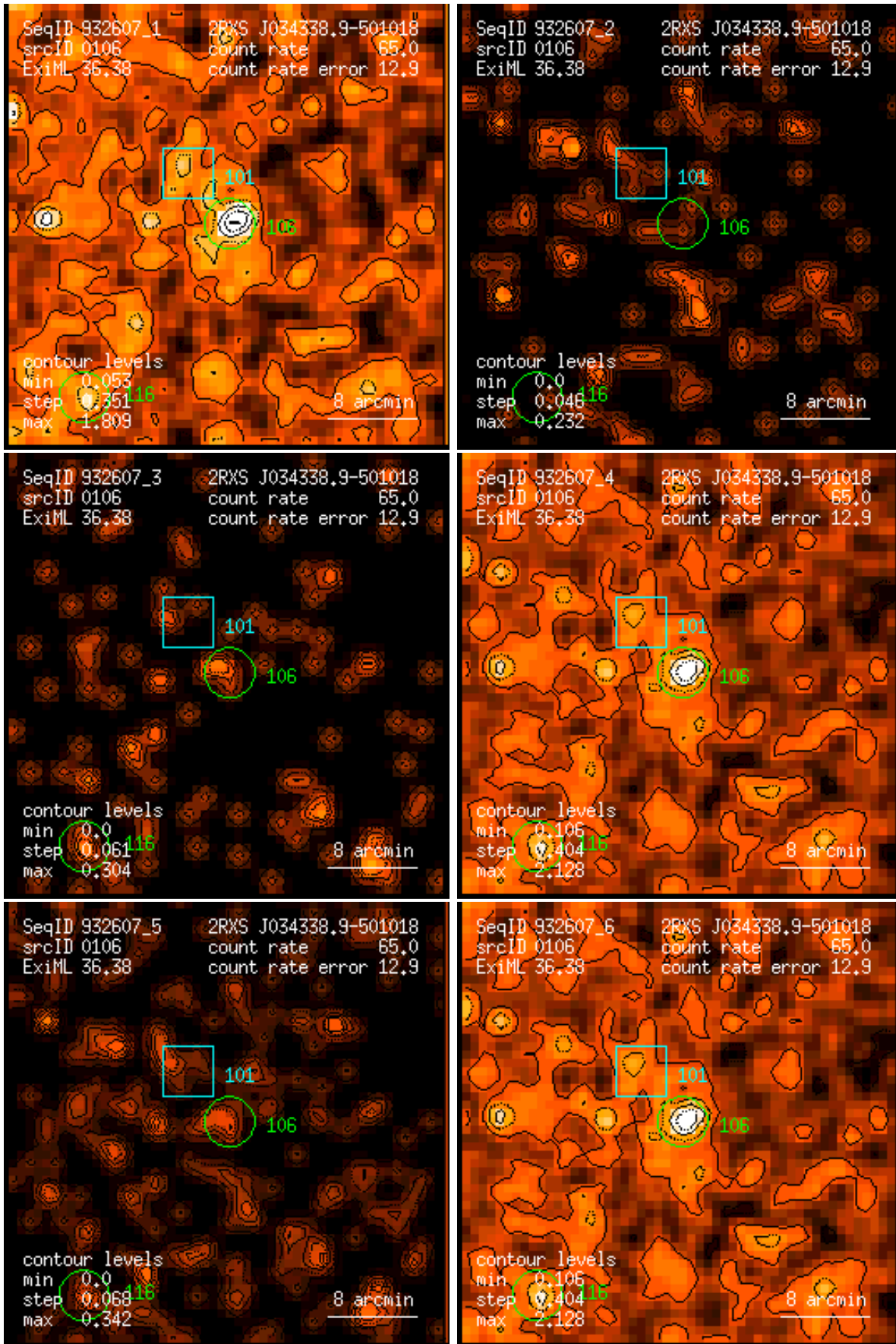
Figure 106: RASS 932607: detection 0106: band rate images, Gaussian filter: (1) PSPC channels 11 – 41, (2) 52 – 90, (3) 91 – 201, (4) 11 – 235, (5) 52 – 201, (6) 11 – 201. Broad band rates in counts/ks. Band rate contour levels in counts/ks/arcmin 2 .
