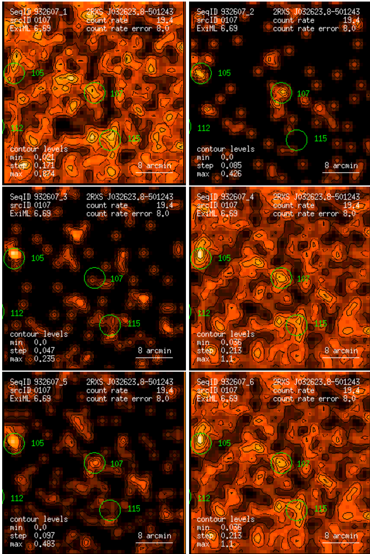
Figure 107: RASS 932607: detection 0107: band rate images, Gaussian filter: (1) PSPC channels 11 – 41, (2) 52 – 90, (3) 91 – 201, (4) 11 – 235, (5) 52 – 201, (6) 11 – 201. Broad band rates in counts/ks. Band rate contour levels in counts/ks/arcmin 2 .
