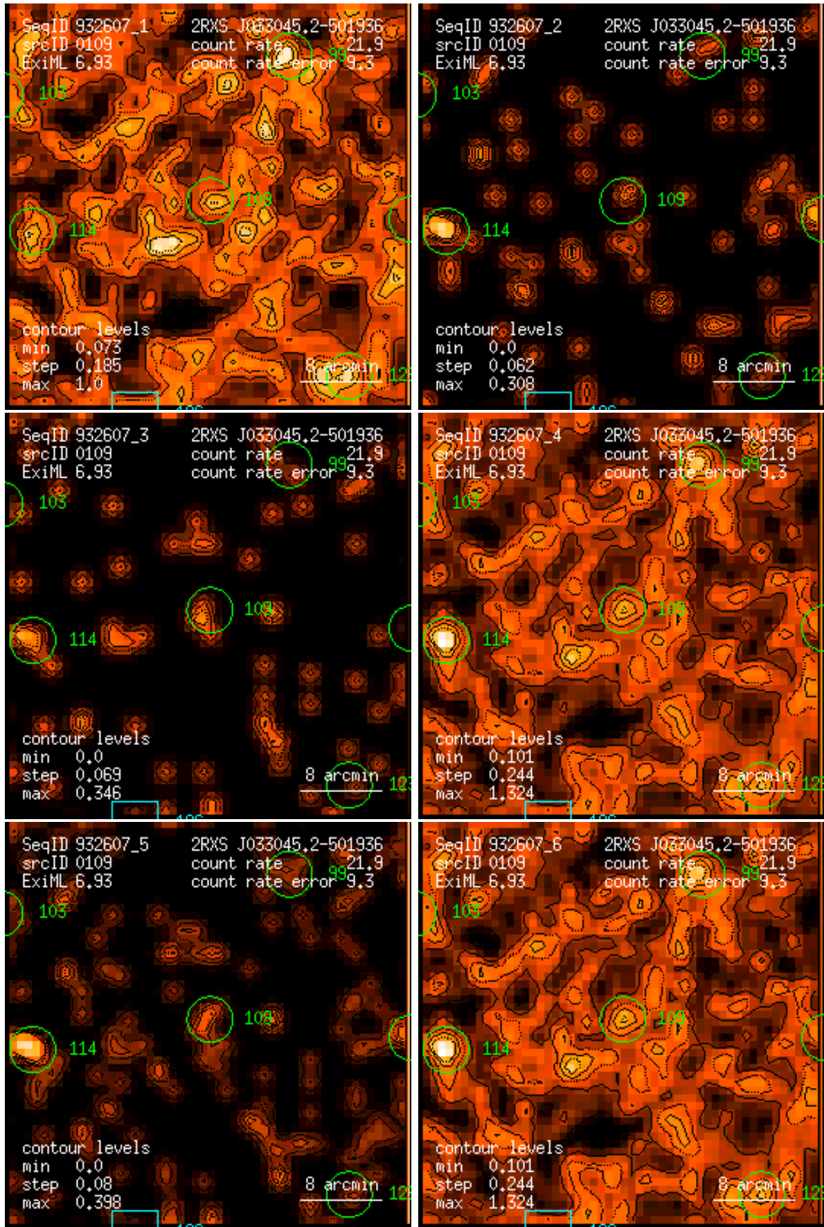
Figure 109: RASS 932607: detection 0109: band rate images, Gaussian filter: (1) PSPC channels 11 – 41, (2) 52 – 90, (3) 91 – 201, (4) 11 – 235, (5) 52 – 201, (6) 11 – 201. Broad band rates in counts/ks. Band rate contour levels in counts/ks/arcmin 2 .
