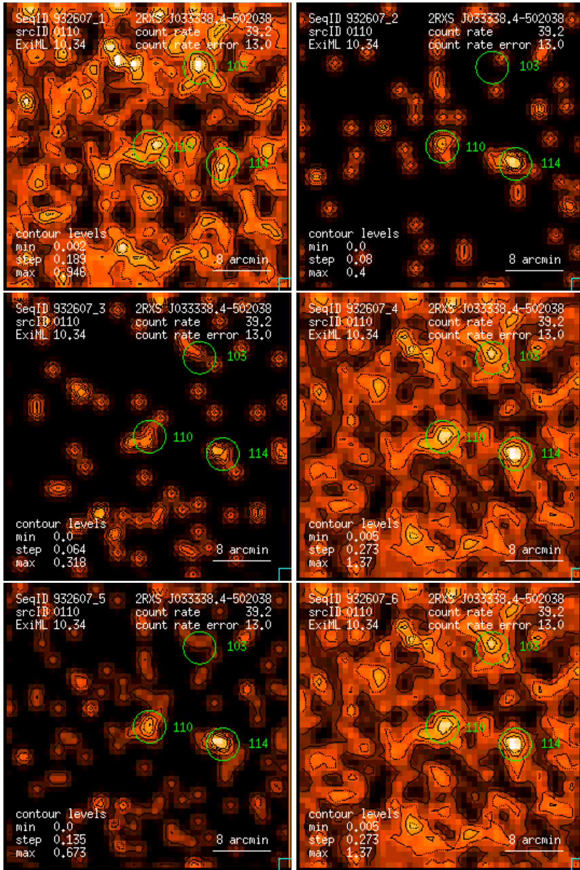
Figure 110: RASS 932607: detection 0110: band rate images, Gaussian filter: (1) PSPC channels 11 – 41, (2) 52 – 90, (3) 91 – 201, (4) 11 – 235, (5) 52 – 201, (6) 11 – 201. Broad band rates in counts/ks. Band rate contour levels in counts/ks/arcmin 2 .
