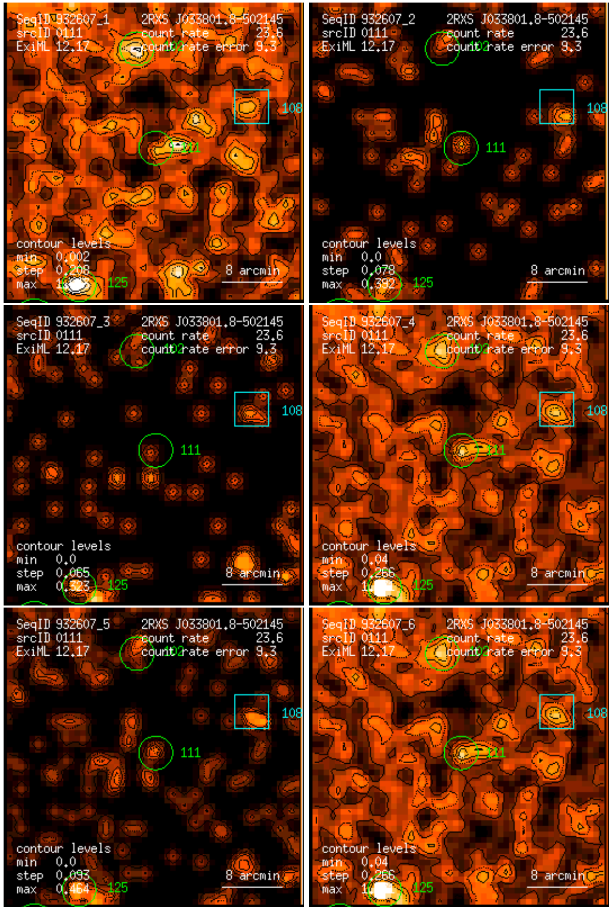
Figure 111: RASS 932607: detection 0111: band rate images, Gaussian filter: (1) PSPC channels 11 – 41, (2) 52 – 90, (3) 91 – 201, (4) 11 – 235, (5) 52 – 201, (6) 11 – 201. Broad band rates in counts/ks. Band rate contour levels in counts/ks/arcmin 2 .
