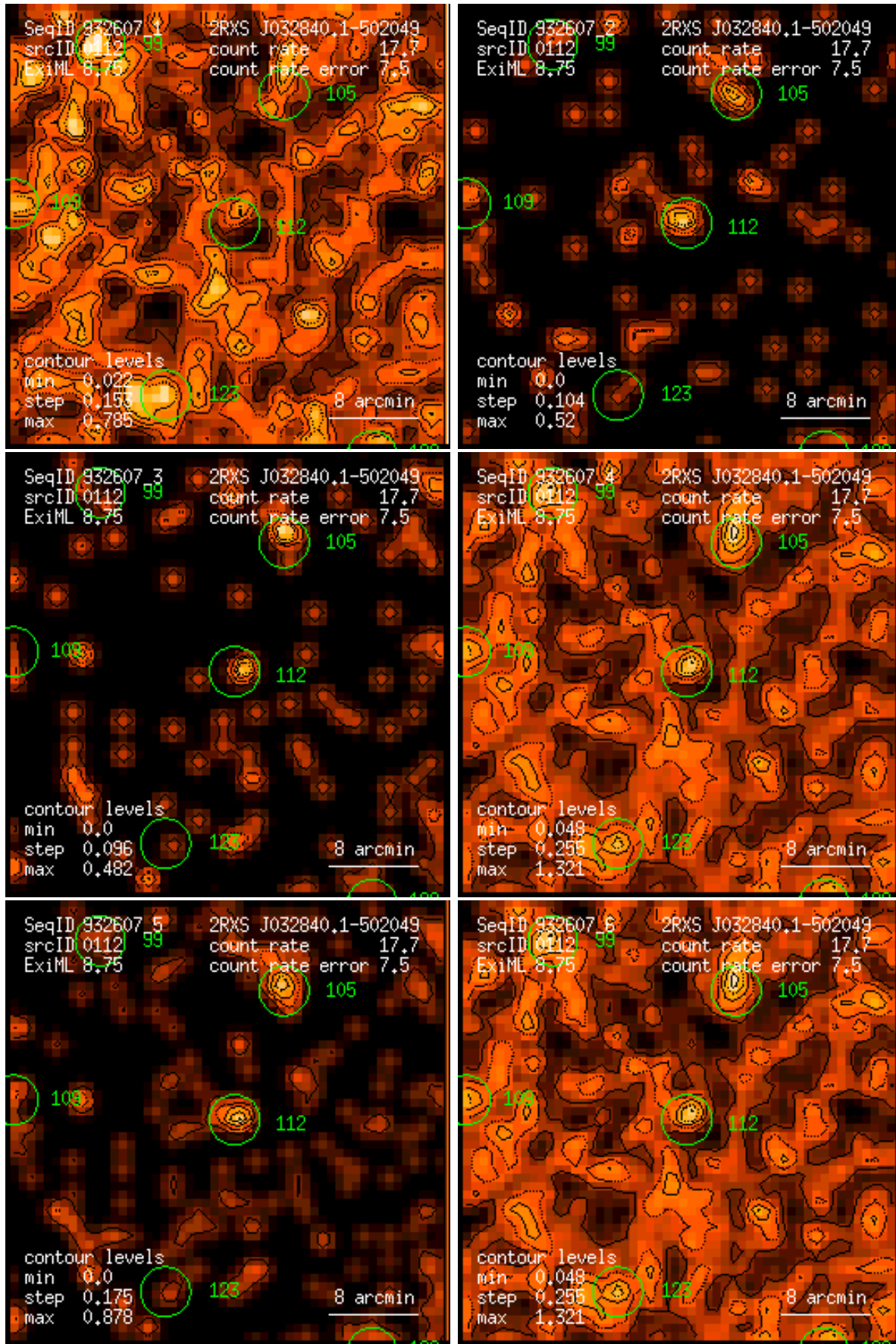
Figure 112: RASS 932607: detection 0112: band rate images, Gaussian filter: (1) PSPC channels 11 – 41, (2) 52 – 90, (3) 91 – 201, (4) 11 – 235, (5) 52 – 201, (6) 11 – 201. Broad band rates in counts/ks. Band rate contour levels in counts/ks/arcmin 2 .
