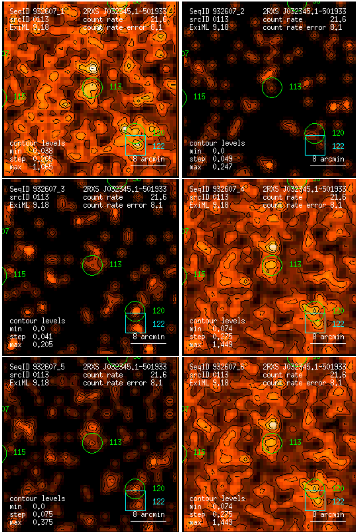
Figure 113: RASS 932607: detection 0113: band rate images, Gaussian filter: (1) PSPC channels 11 – 41, (2) 52 – 90, (3) 91 – 201, (4) 11 – 235, (5) 52 – 201, (6) 11 – 201. Broad band rates in counts/ks. Band rate contour levels in counts/ks/arcmin 2 .
